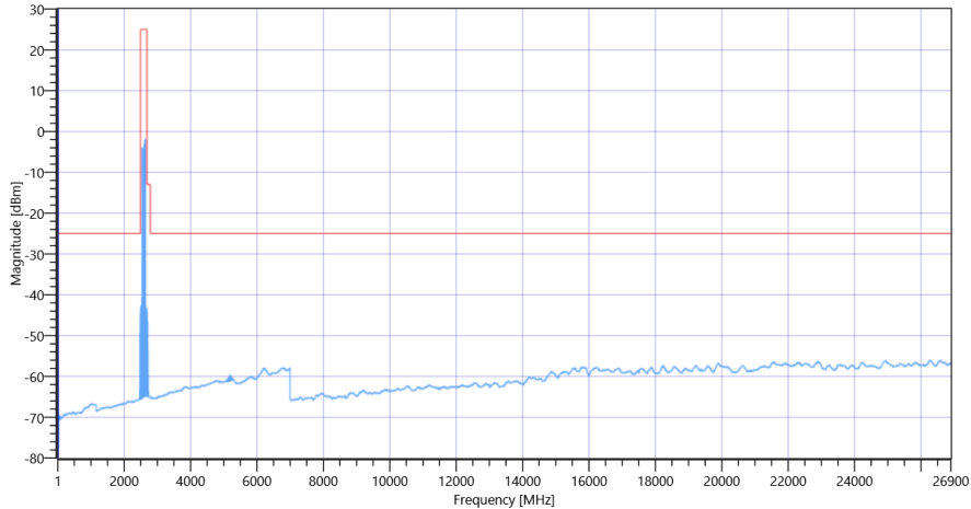
FCC, ISED # TX Emissions conducted ~ NR Band_41 Ant-1 SCS-30 2592.99 MHz
