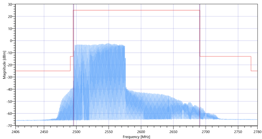
FCC, ISED # TX Emissions conducted ~ NR Band_41 Ant-1 SCS-30 2536.02
