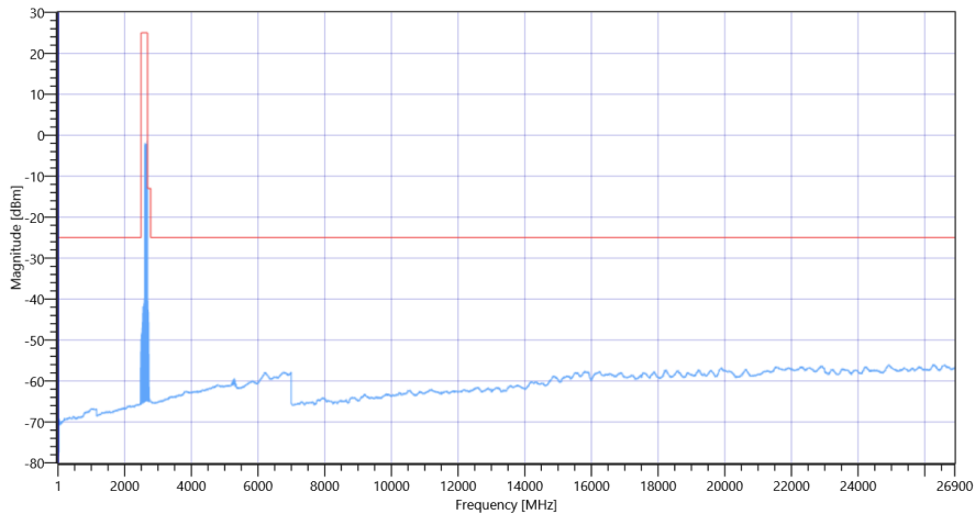
FCC, ISED # TX Emissions conducted ~ NR Band_41 Ant-1 SCS-30 2644.98 MHz
