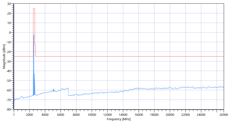
FCC, ISED # TX Emissions conducted ~ NR Band_41 Ant-1 SCS-30 2536.02 MHz
