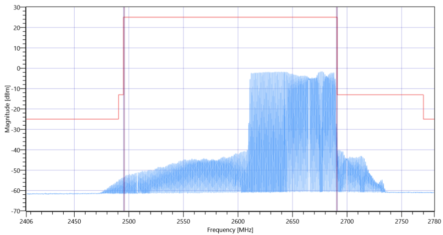
FCC, ISED # TX Emissions conducted ~ NR Band_41 Ant-1 SCS-30 2649.99
