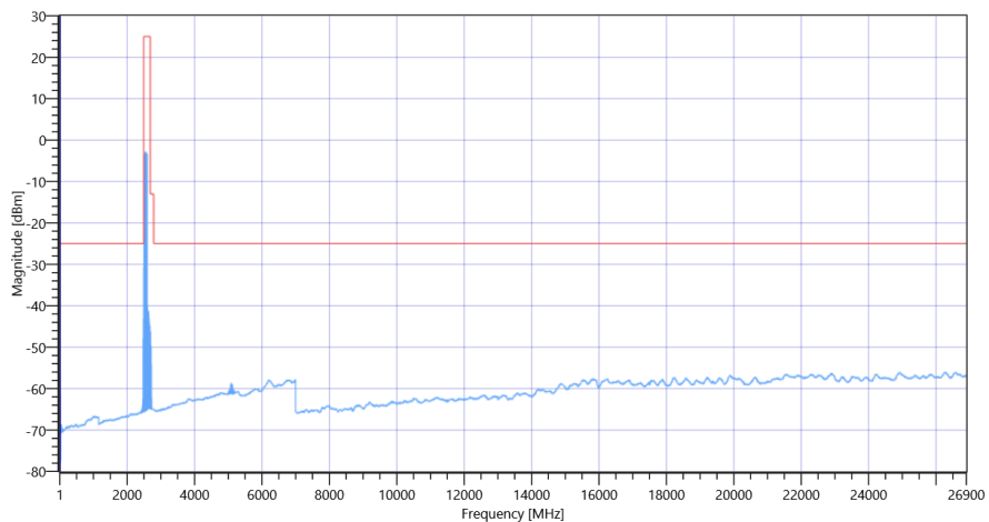
FCC, ISED # TX Emissions conducted ~ NR Band_41 Ant-1 SCS-30 2546.01 MHz
