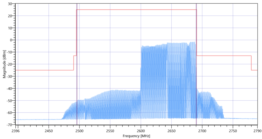
FCC, ISED # TX Emissions conducted ~ NR Band_41 Ant-1 SCS-30 2644.98
