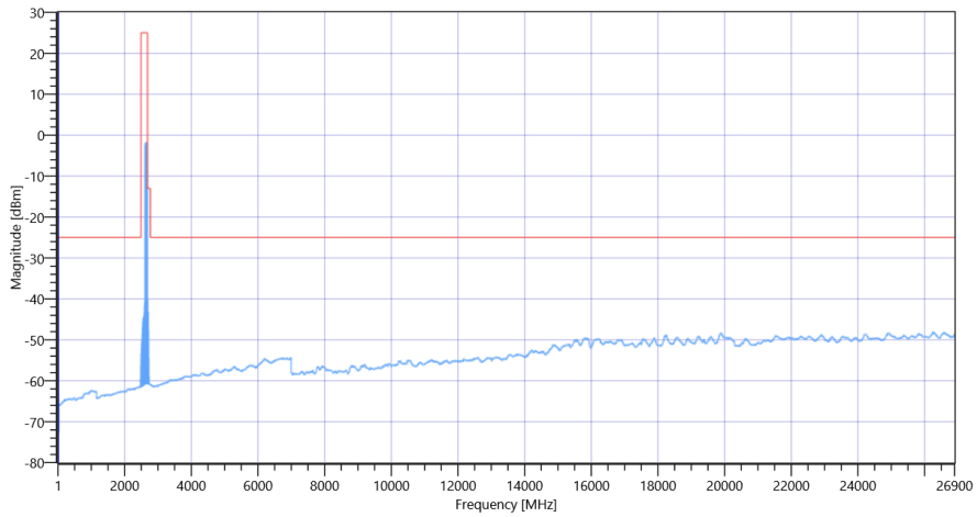
FCC, ISED # TX Emissions conducted ~ NR Band_41 Ant-1 SCS-30 2649.99 MHz
