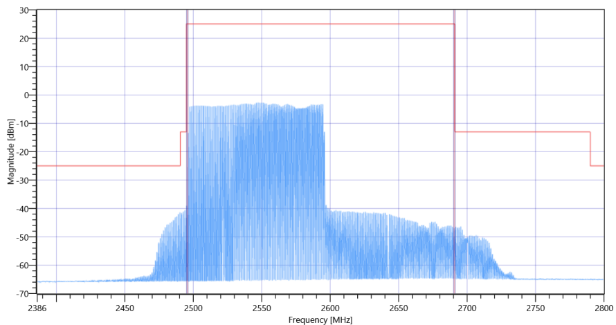
FCC, ISED # TX Emissions conducted ~ NR Band_41 Ant-1 SCS-30 2546.01
