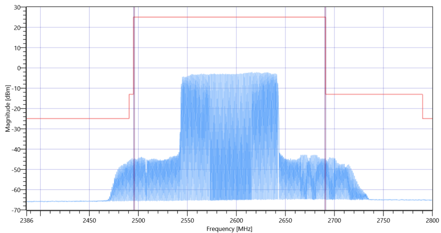
FCC, ISED # TX Emissions conducted ~ NR Band_41 Ant-1 SCS-30 2592.99
