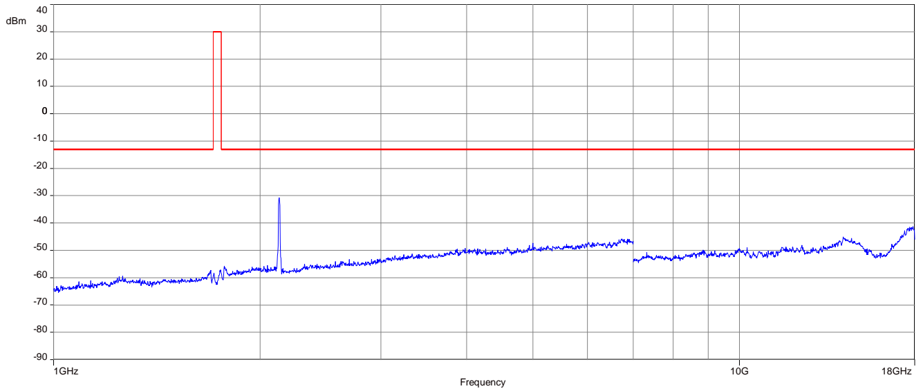
Carrier notched with 1.73 GHz rejection filter
