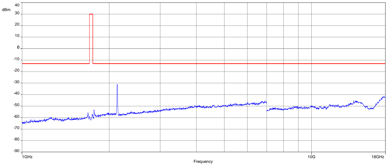
Plot 6: 16-QAM - Middle channel (1 GHz – 18 GHz)
