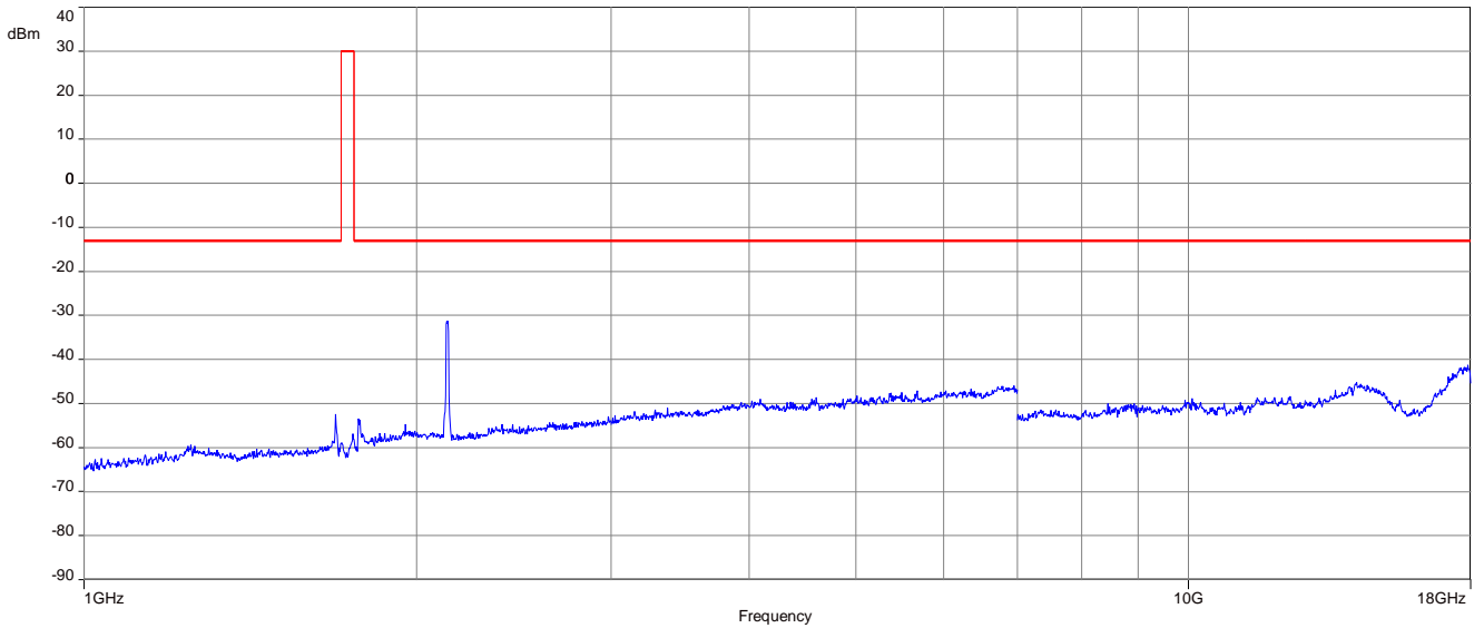
Carrier notched with 1.73 GHz rejection filter
