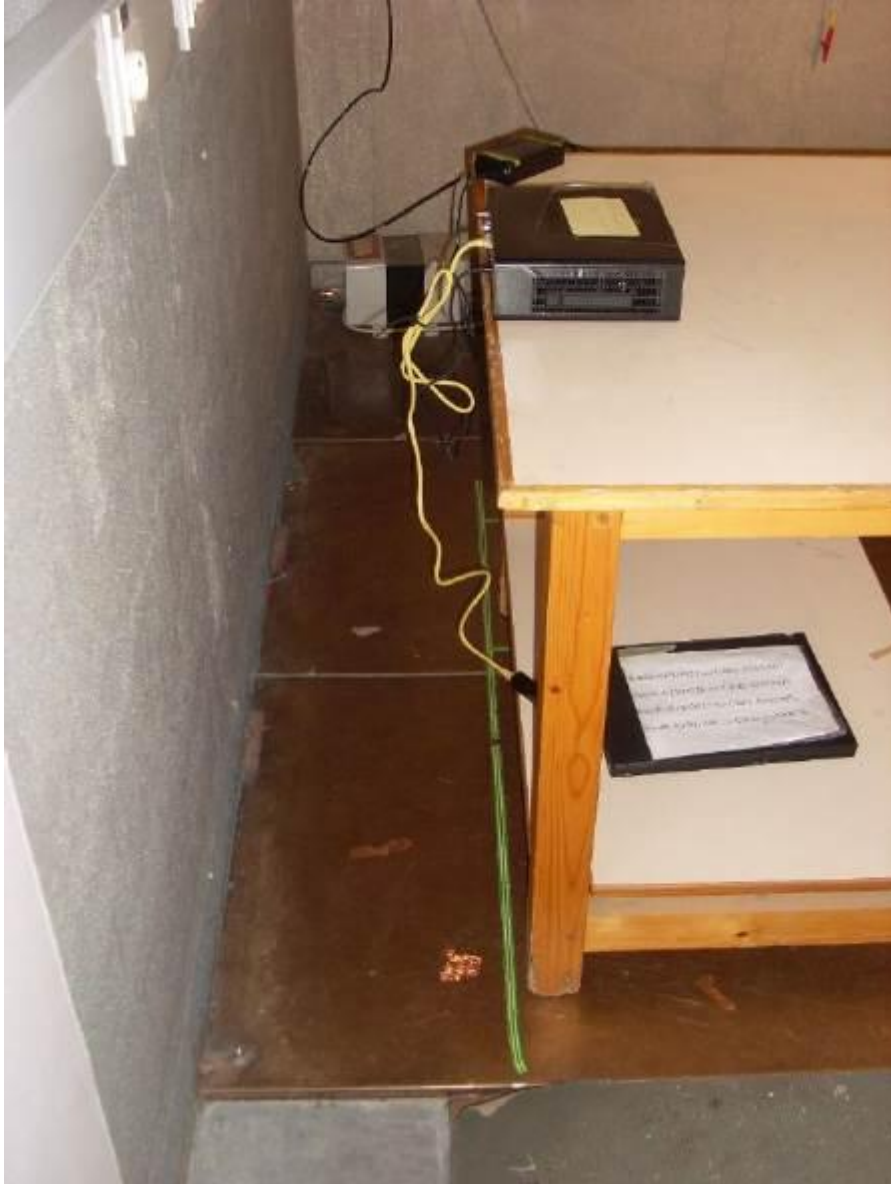
Test setup for power line conducted emissions
