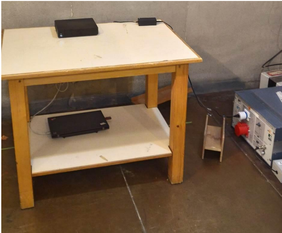
Test setup for power line conducted emissions
