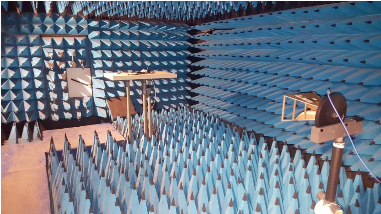
Test setup for radiated field strength ( f > 1\text{GHz} )
