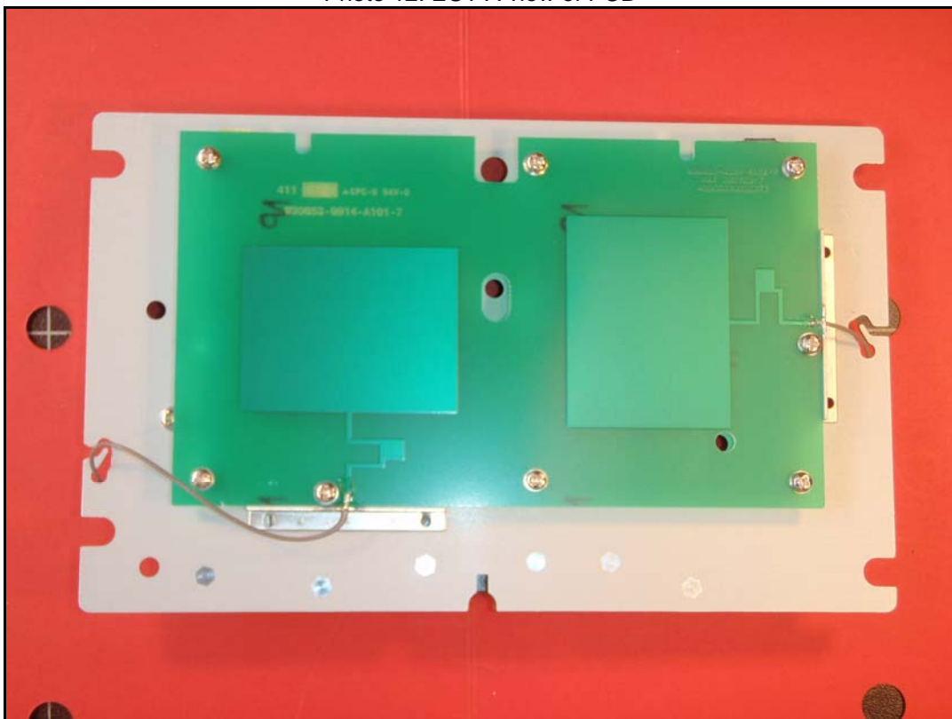
Photo 12: EUT A view of PCB
