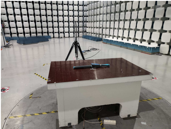
Radiated Emissions Below 30 MHz
