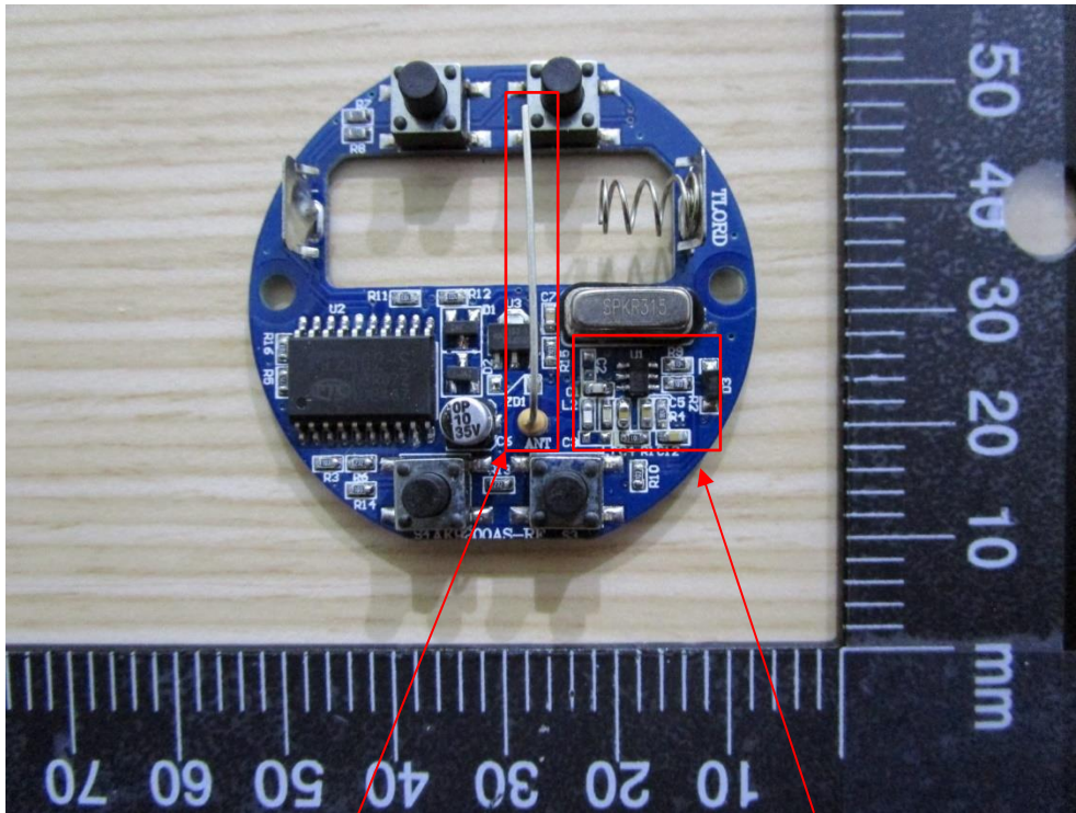
RF Antenna
