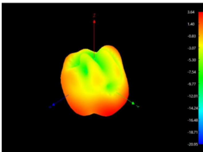
Radiation Pattern For 915MHz Antenna
