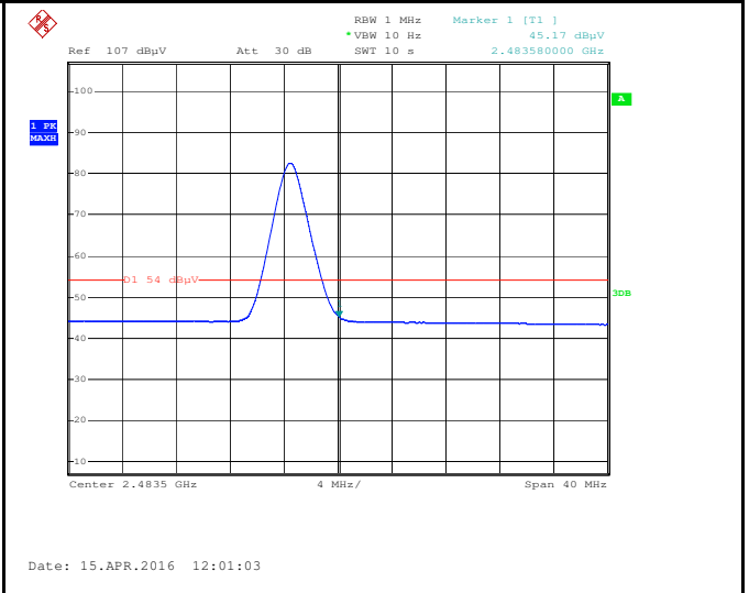
Band Edge, Right Side (Average)
