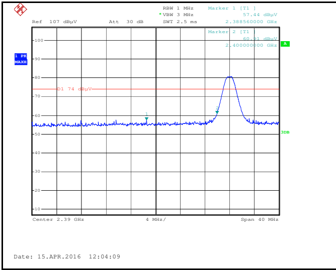
Band Edge, Left Side (Peak) Note: F1 is frequency 2390MHz; F2 is frequency 2400MHz
