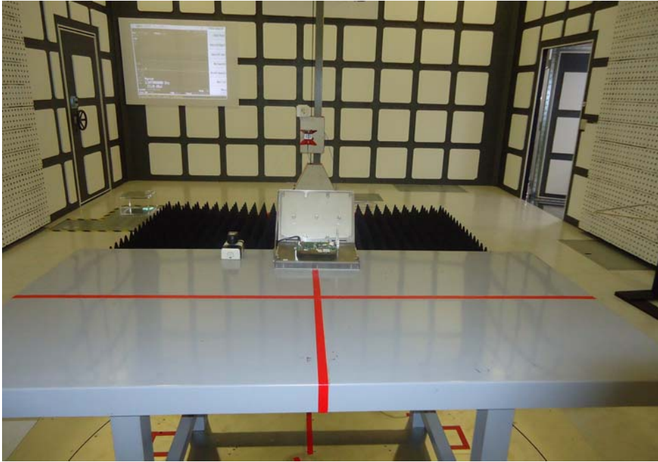
Mode 1 / Mode 2 / Mode 3 / Mode 4 _ Above 1GHz _ Rear View
