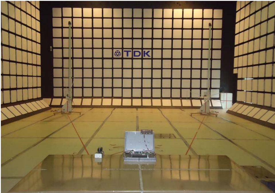
Mode 5 _ Below 1GHz _ Rear View
