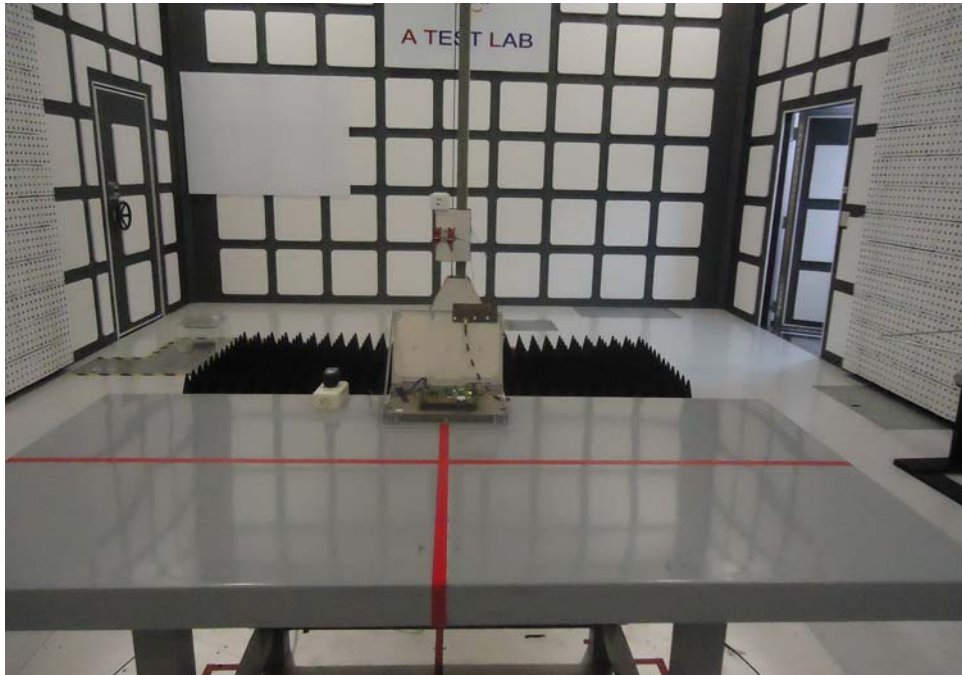
Mode 5 _ Above 1GHz _ Rear View
