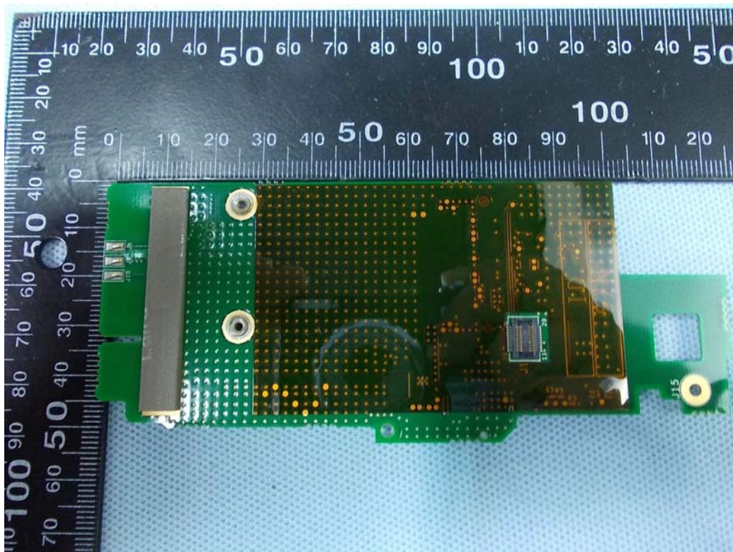
16. Rear view of PCB1
