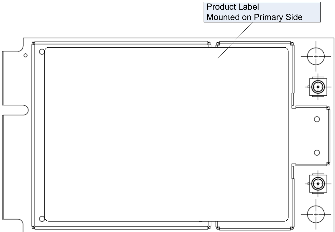
Figure 1 Ericsson F3507g Label Location
