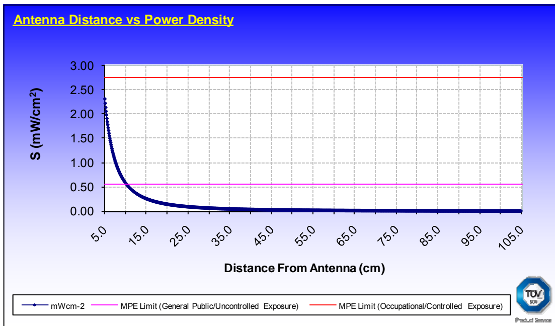
Figure 5 - This graph shows the S field (mW/cm²) strength value with regards to distance from the Antenna (cm)
