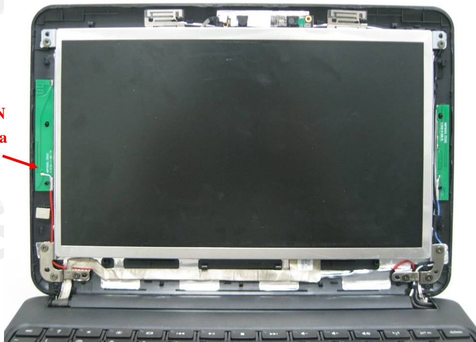
Fig.8 Antenna position of EUT
