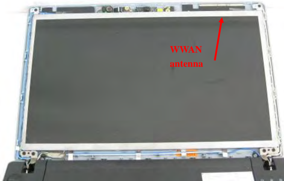
Fig.3 Antenna position of EUT
