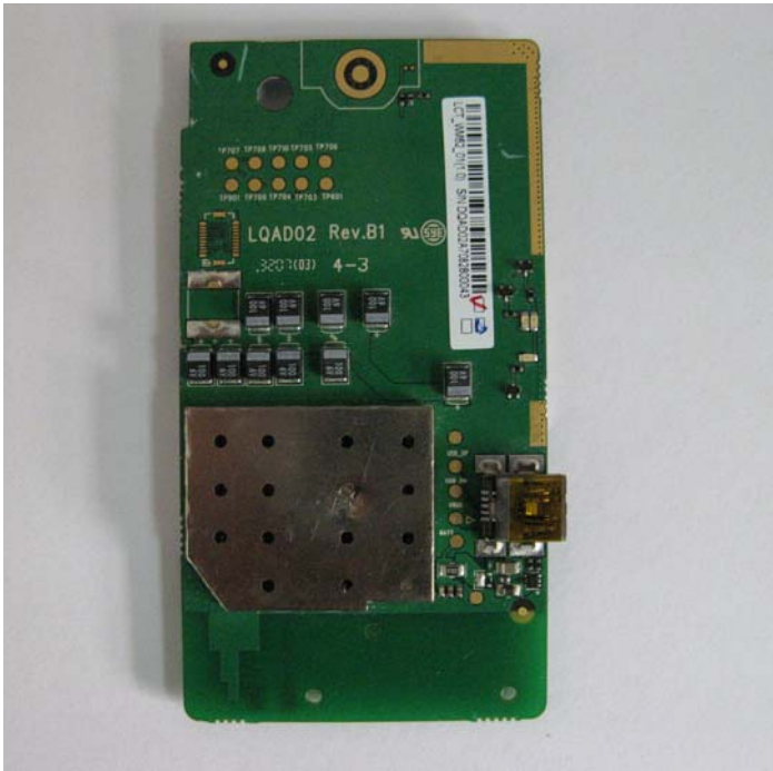
Picture 3: the top view of the sample with the RF shield-1
