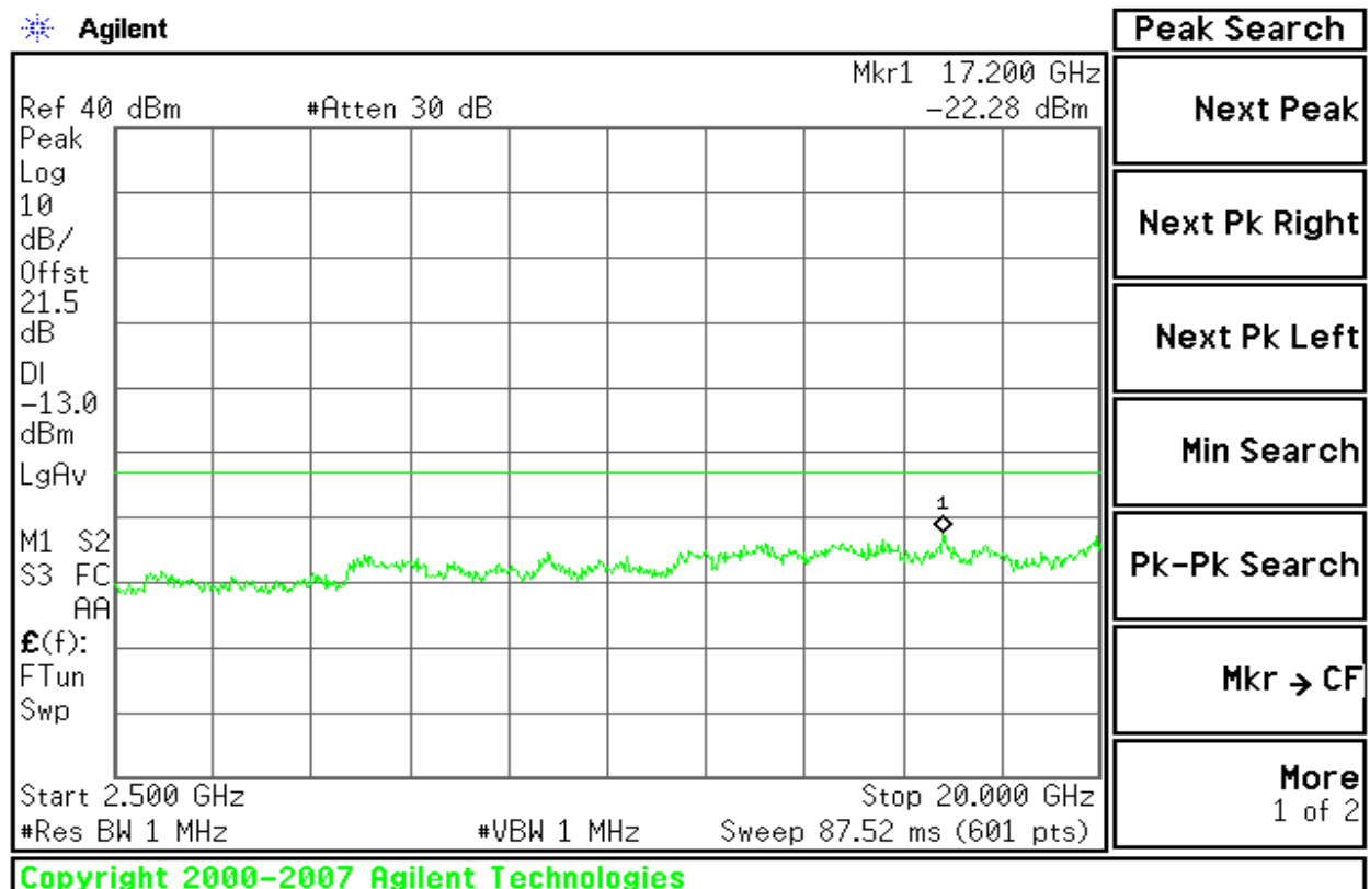
Figure 8-4: Out of Band emission at antenna terminals –EDGE CH Mid
