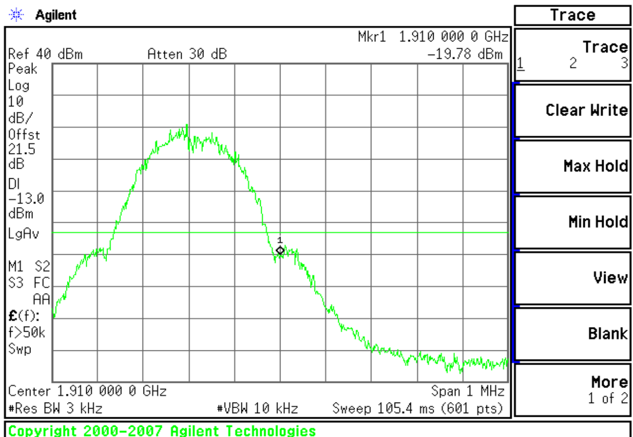
Figure 10-2: Band Edge emissions – GPRS CH High
