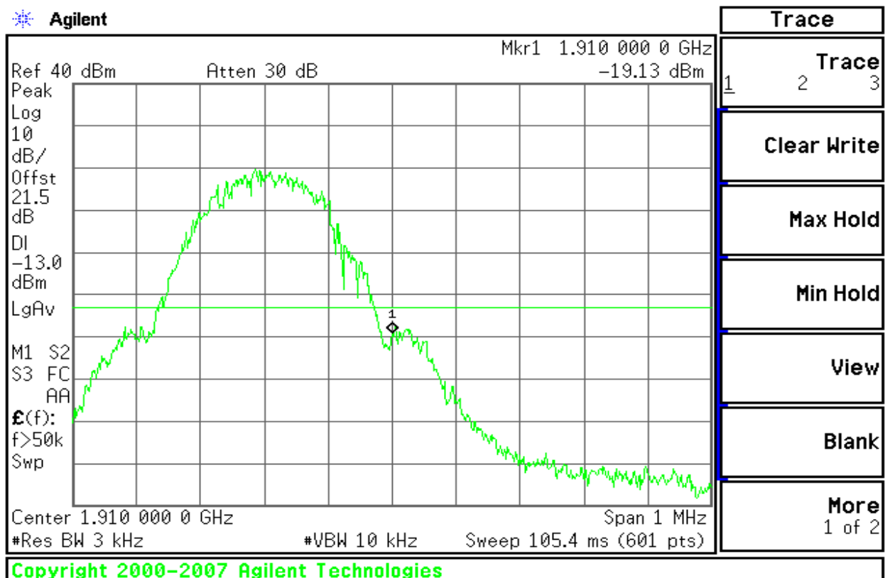
Figure 10-2: Band Edge emissions – EDGE CH High
