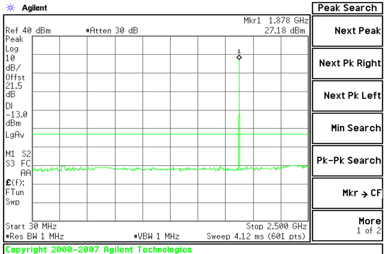
Figure 8-4: Out of Band emission at antenna terminals –EDGE CH Mid
