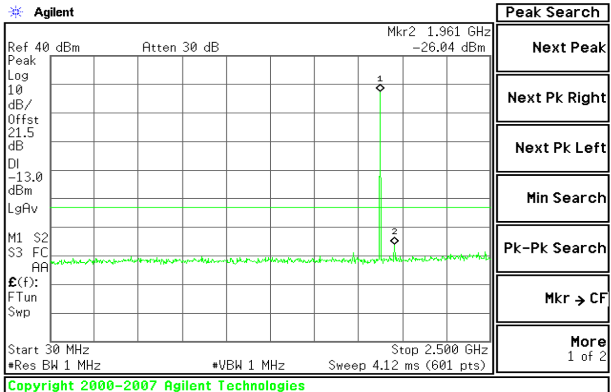
Figure 8-4: Out of Band emission at antenna terminals –GPRS CH Mid
