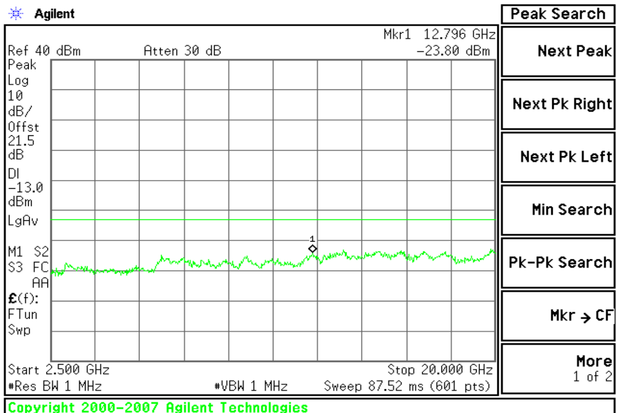
Figure 8-4: Out of Band emission at antenna terminals –GPRS CH Mid
