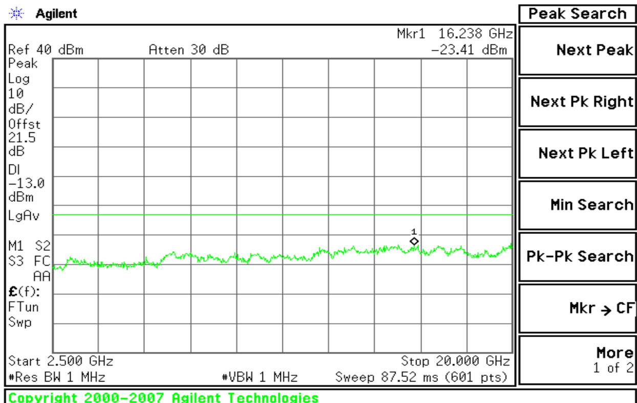
Figure 8-2: Out of Band emission at antenna terminals –EDGE CH Low
