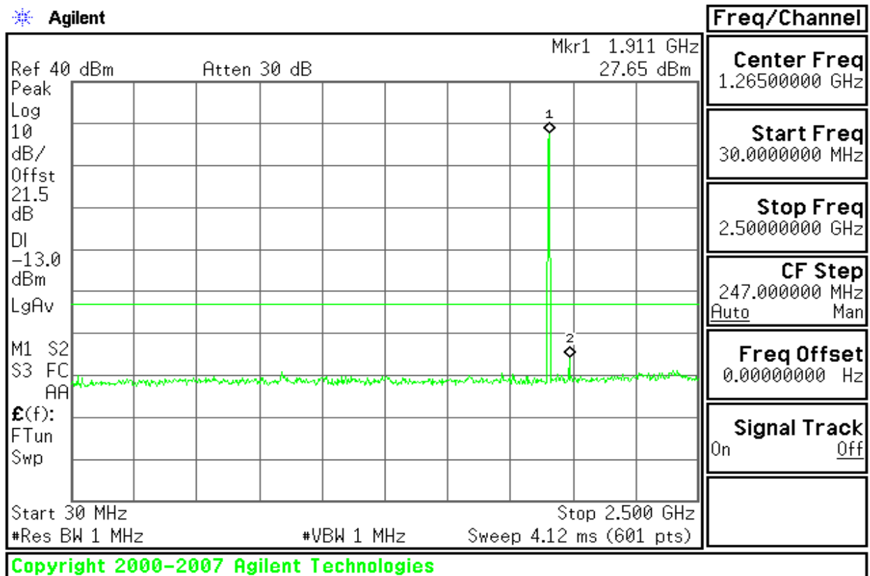
Figure 8-5: Out of Band emission at antenna terminals –EDGE CH High
