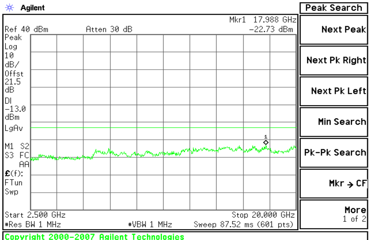
Figure 8-6: Out of Band emission at antenna terminals –EDGE CH High
