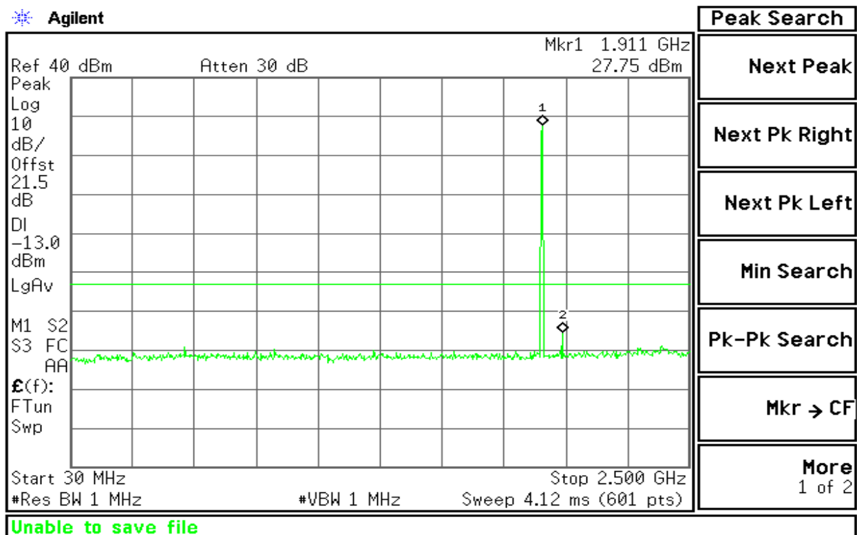
Figure 8-5: Out of Band emission at antenna terminals –GPRS CH High
