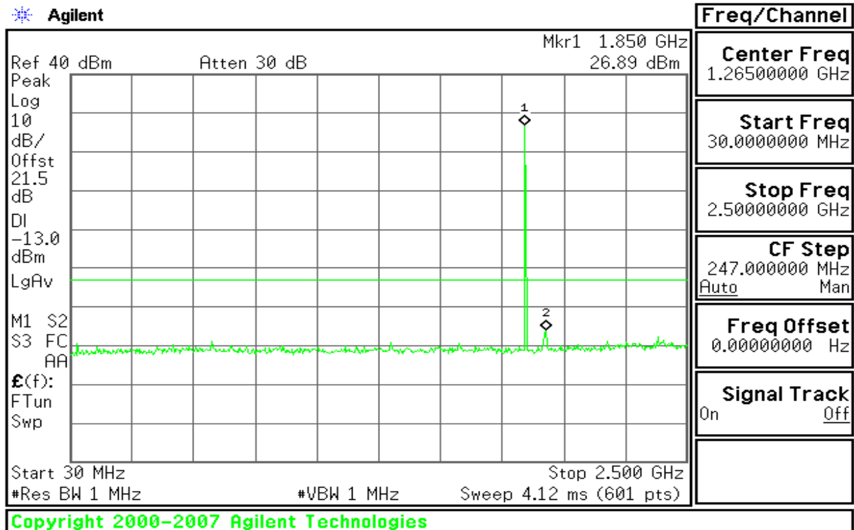
Figure 8-2: Out of Band emission at antenna terminals –GPRS CH Low
