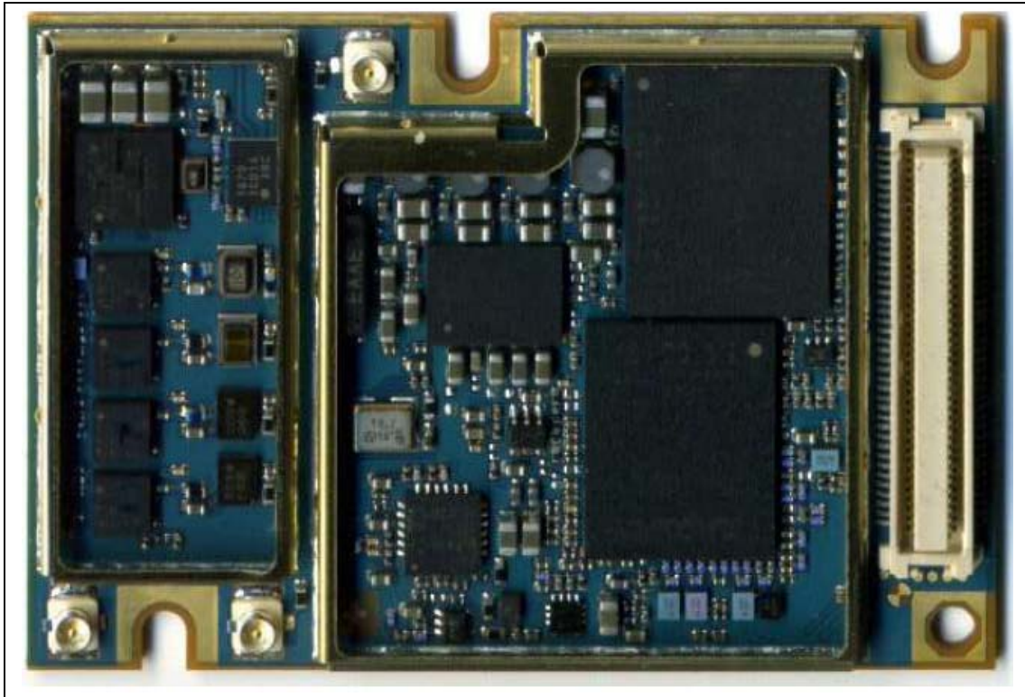
GSM/WCDMA Board Front
