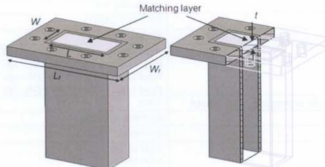
Figure 1: Validation Waveguide Dimensions
