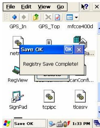
Figure 4. Registry Save
