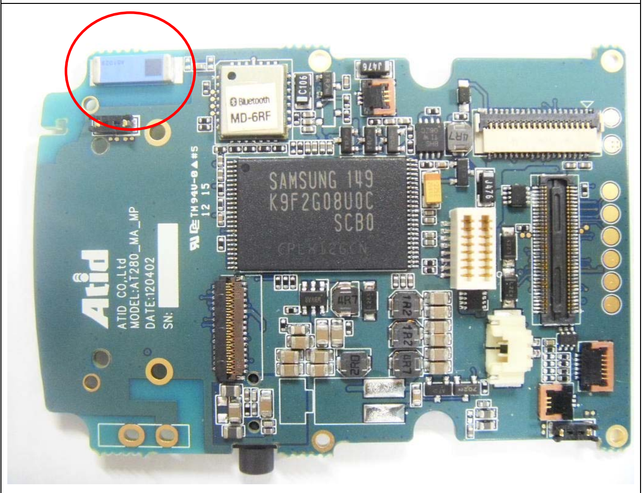
ANTENNA- M/N: ALA931C5
