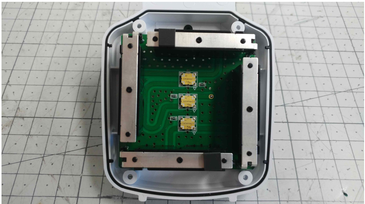
RFID Antenna Board Front
