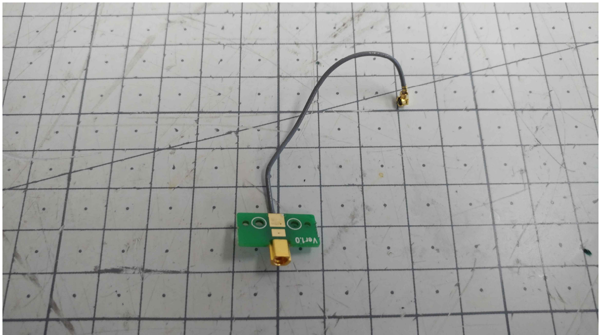
RFID Connector board Front
