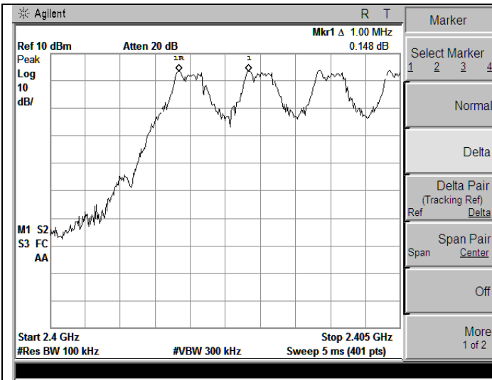
Test Plot of Frequency Separation (1Mbps)
