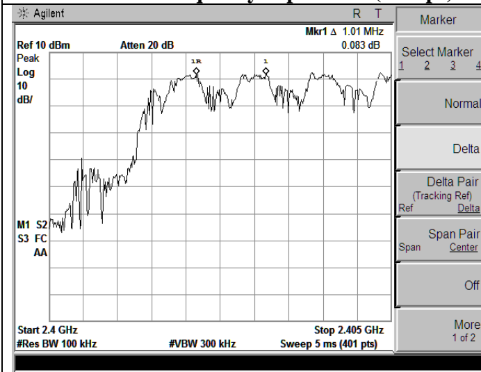
Test Plot of Frequency Separation (3Mbps)
