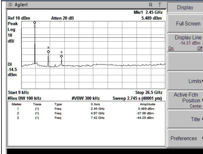
9KHz-26.5GHz High Channel(GFSK)
