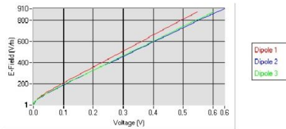
Calibration curves
