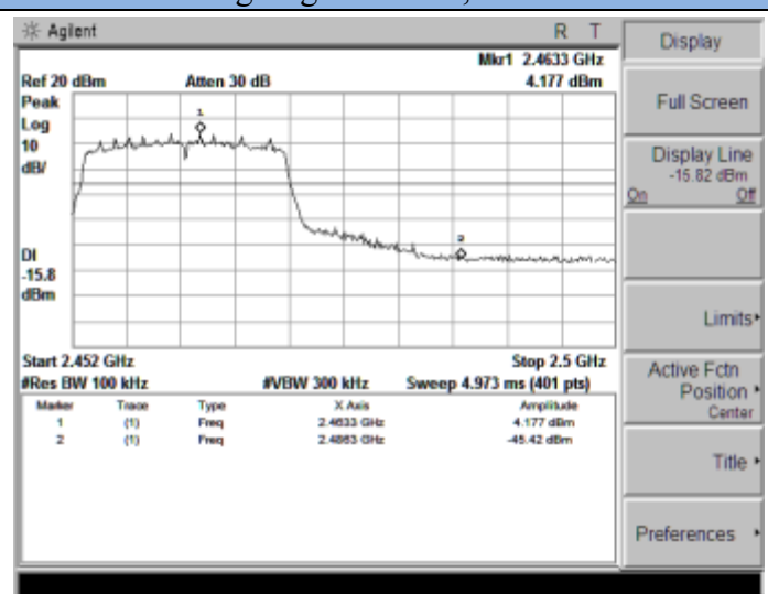
802.11n-HT20-High Channel, 2462MHz
