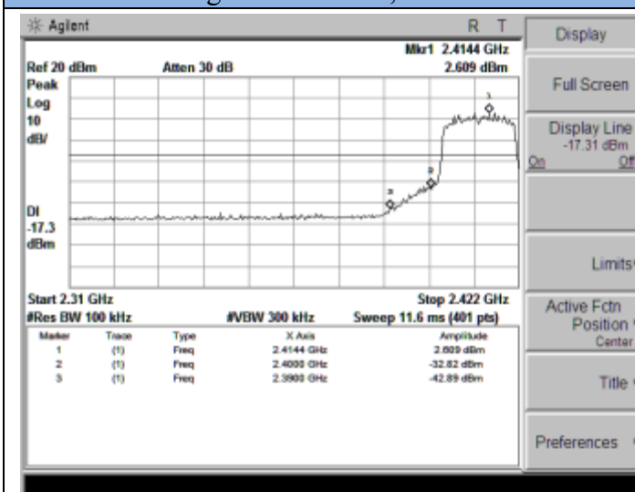
802.11n-HT20-Low Channel, 2412MHz
