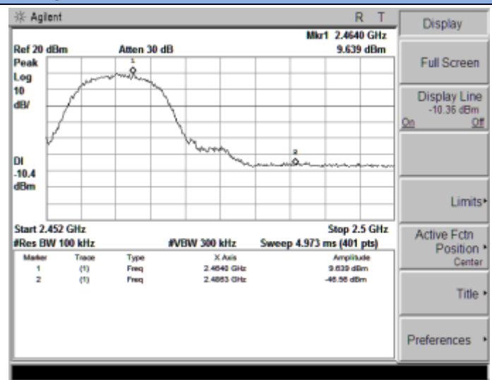
802.11b-High Channel, 2462MHz
