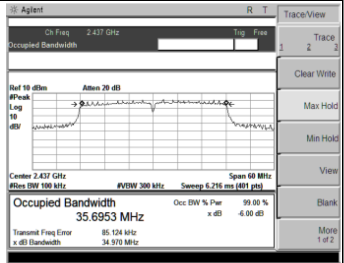
802.11n-HT40-Middle Channel, 2437MHz
