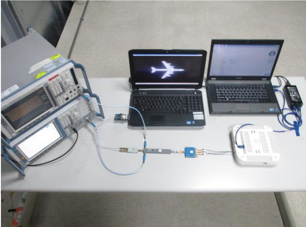
DFS Test
