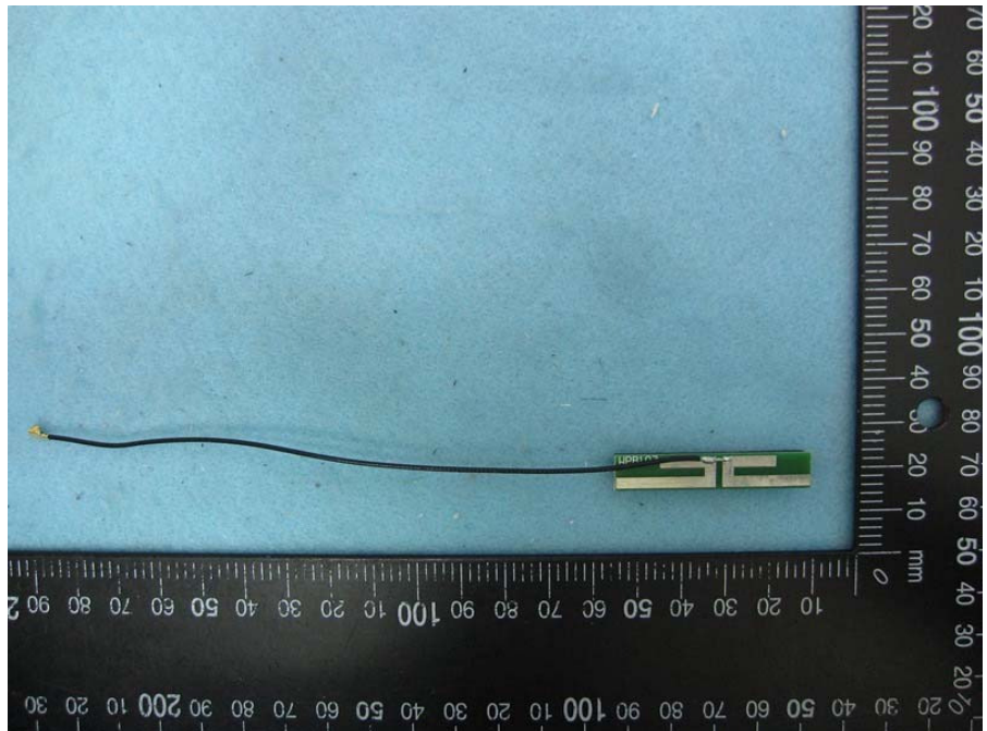
Antenna 5 Part No.: 1415-0172000
