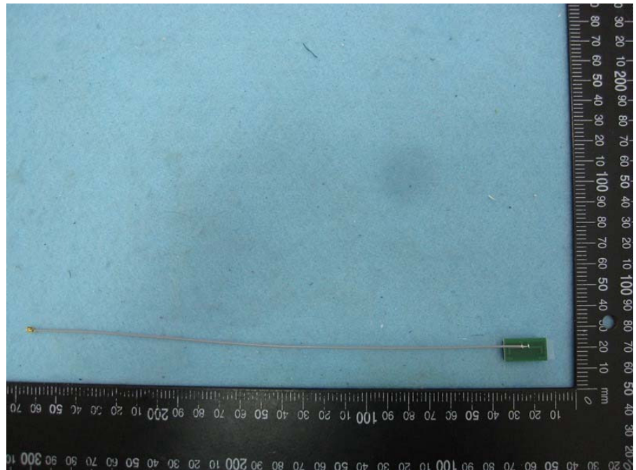
Antenna 2 Part No.: 1415-00XS000
