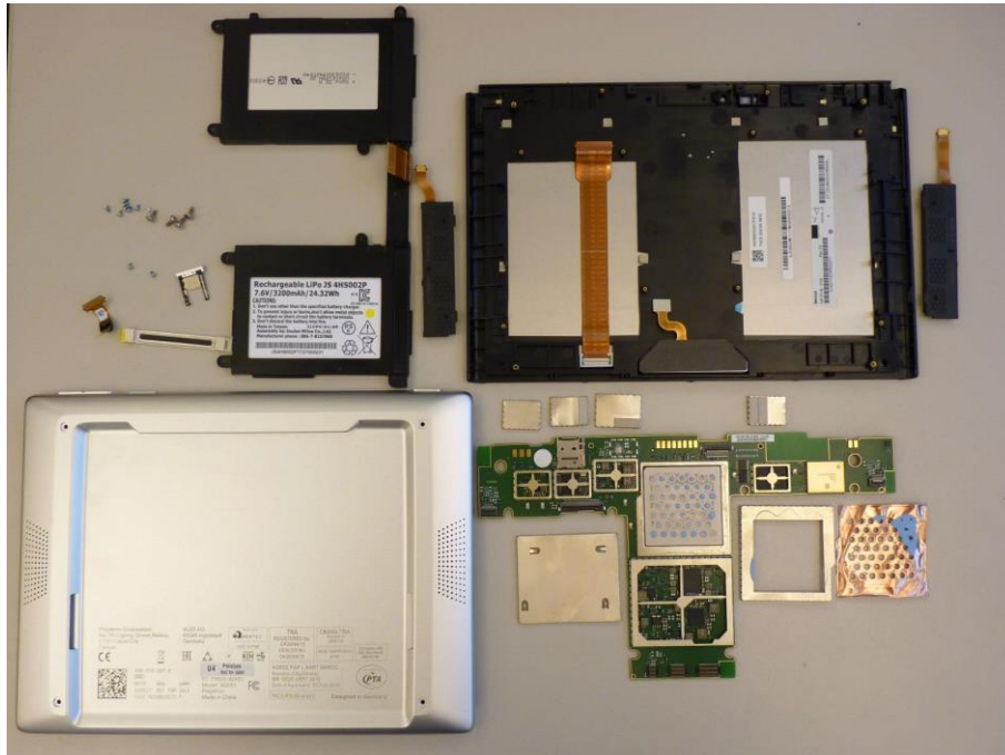
Photo 9: Overview with back cover
