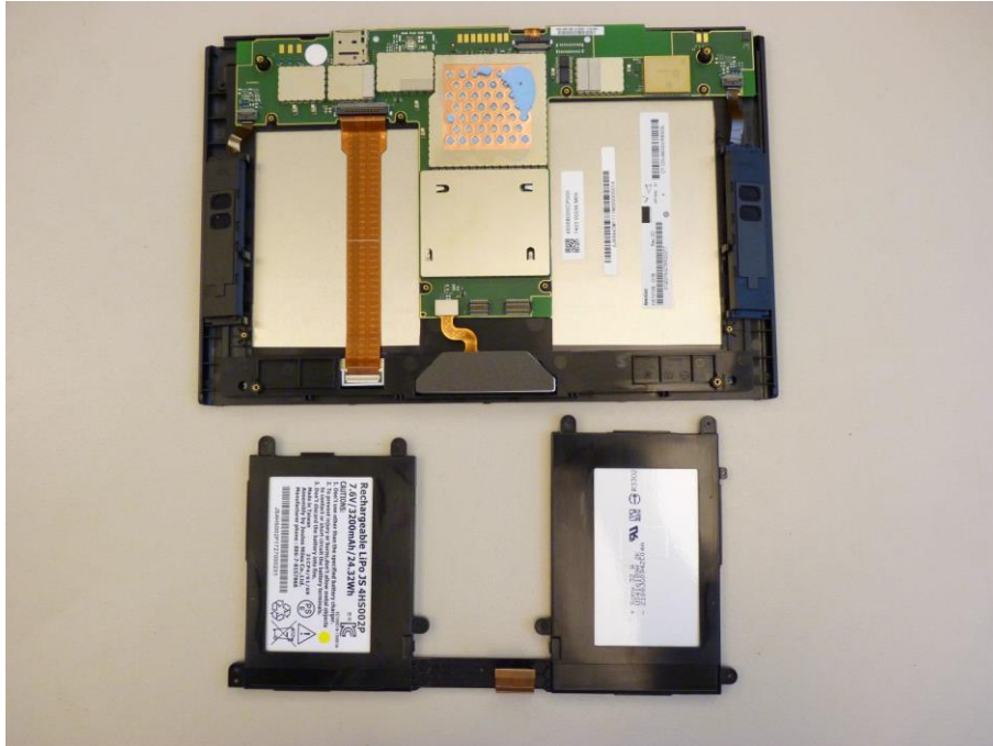
Photo 3: Back cover removed
