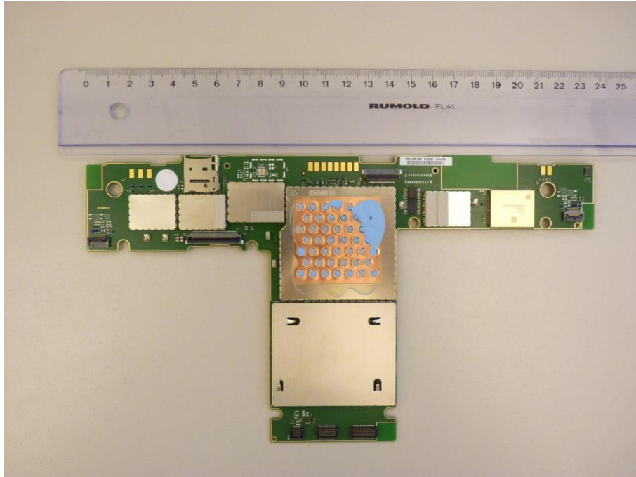
Photo 5: PCB 1 with shieldings
