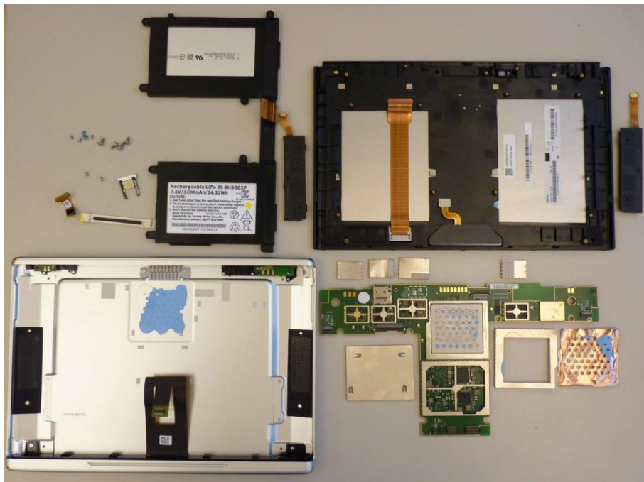
Photo 8: Overview with front cover
