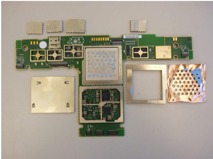
Photo 6: PCB 1 with shieldings removed
