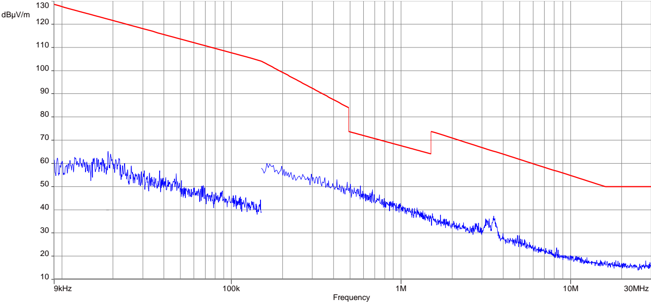
Plot 1: 9 kHz to 30 MHz, channel 39, transmit mode
