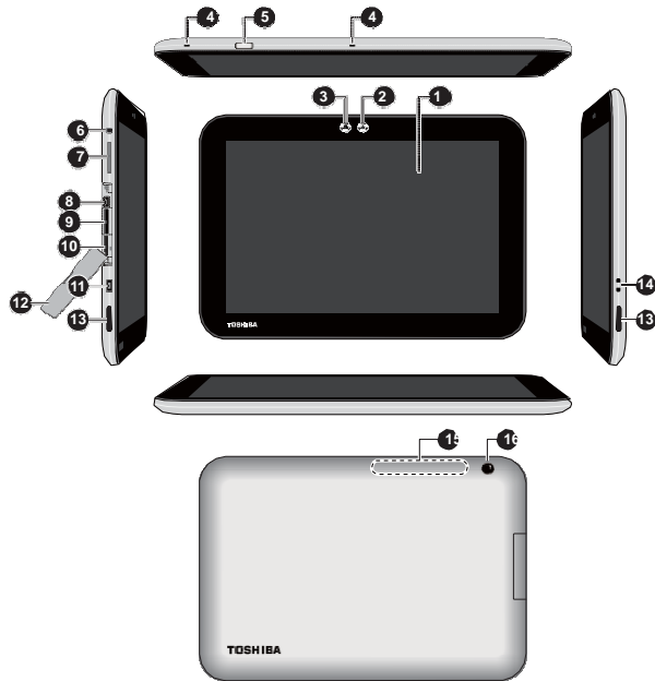
Figure 3-1 Grand tour of the tablet
