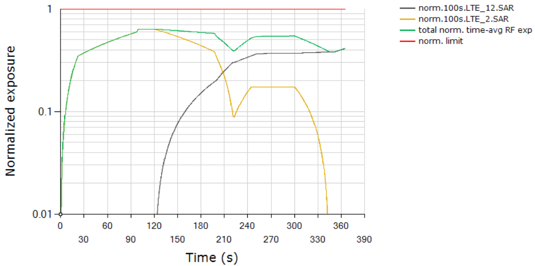
Total Normalized Time-averaged RF Exposure Tech: LTE, Band 12 / Tech: LTE, Band 2
