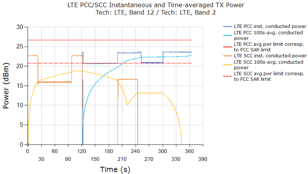
Plot 2: All the conducted Tx power measurement results were converted into time-averaged normalized SAR values using Equation (6a), (6b) and (6c), and plotted below to demonstrate that the time-averaged normalized SAR versus time does not exceed the FCC limit of 1 unit. Equation (6a) is used to convert the LTE Tx power of device to obtain 100s-averaged normalized SAR in LTE UL CA B12 PCC as shown in black curve. Similarly, equation (6b) is used to obtain 100s-averaged normalized SAR in LTE UL CA B2 SCC as shown in orange curve. Equation (6c) is used to obtain total time-averaged normalized SAR as shown in green curve (i.e., sum of black and orange curves).
