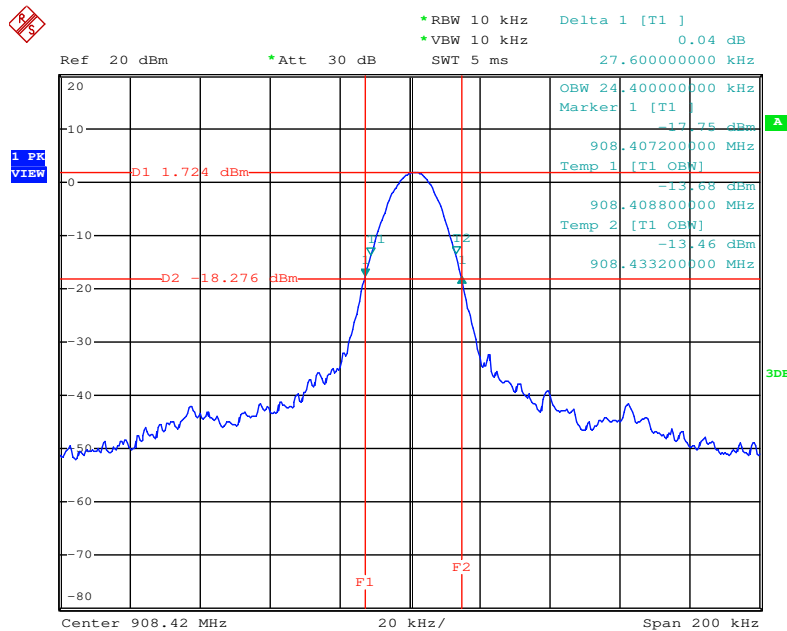
20 dB/99% Bandwidth Plot on 908.42 MHz
