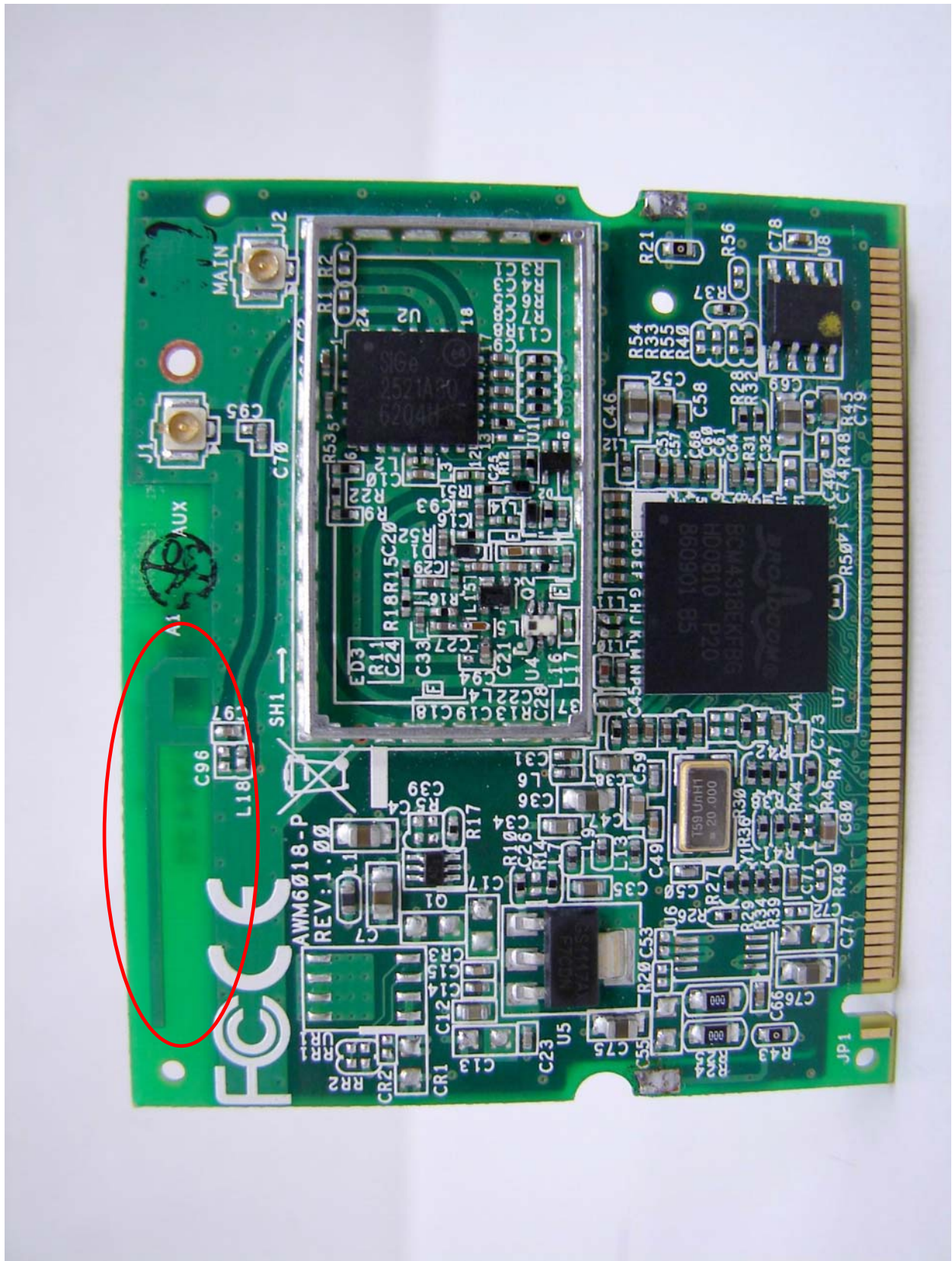
Antenna#2: Printed antenna
