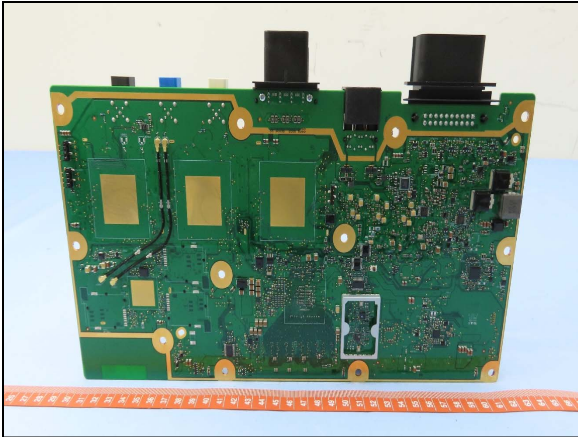
Antenna_LTE/GNSS (Model: 85004261)
