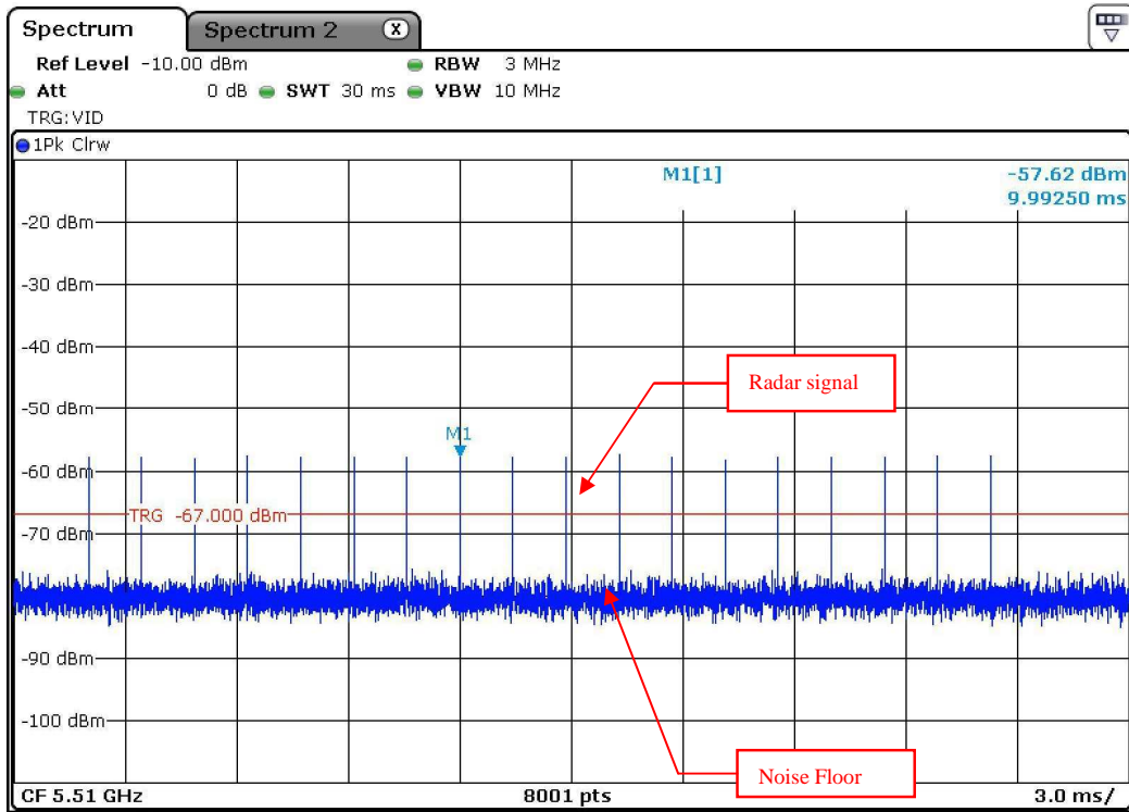
Radar Signal 1
