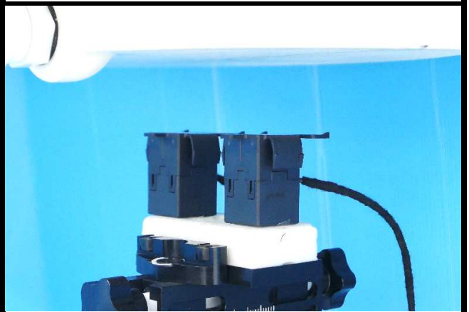
MIMO Top Side of EUT Tested at 41 mm
