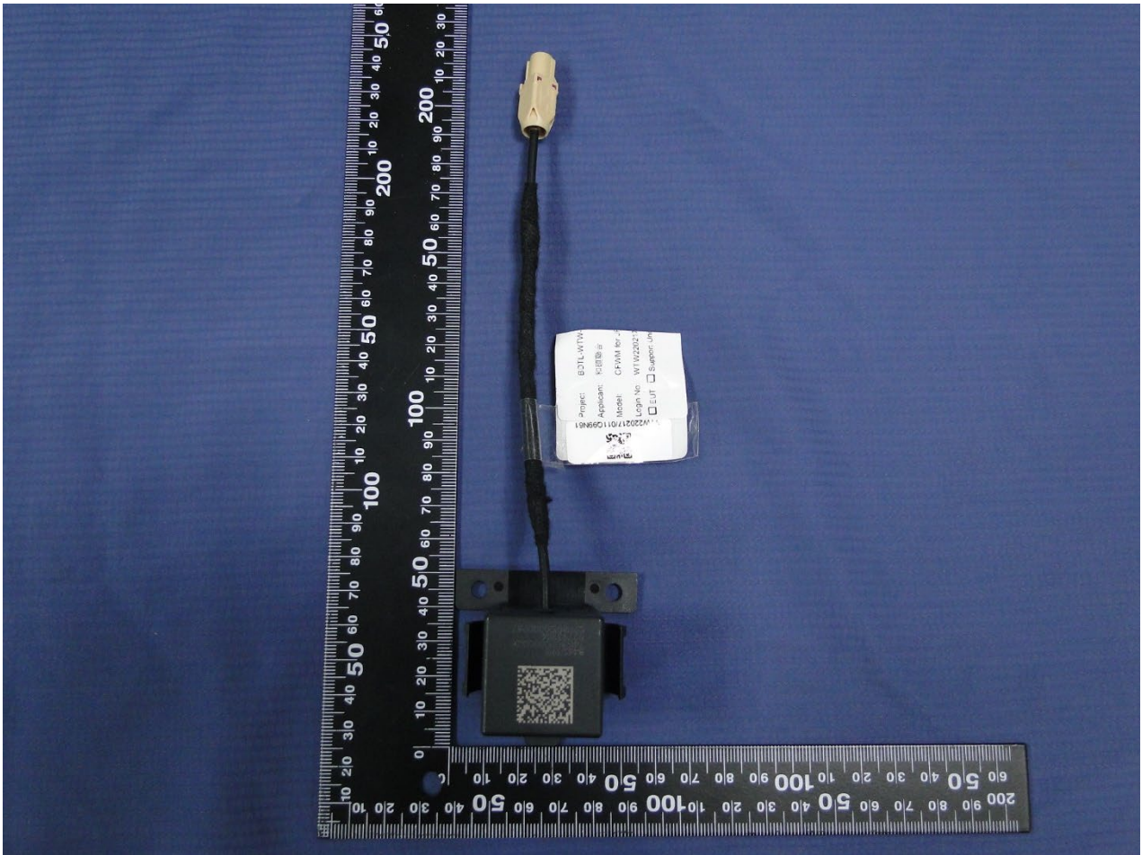
Dimension: L(215mm)*W(54mm)*T(48mm)
