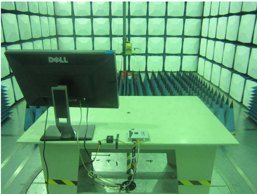
Radiated Emissions Above 1G –Rear View
