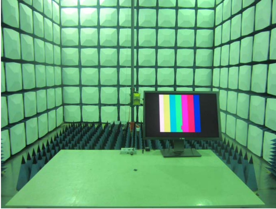
Radiated Emissions Above 1G –Front View
