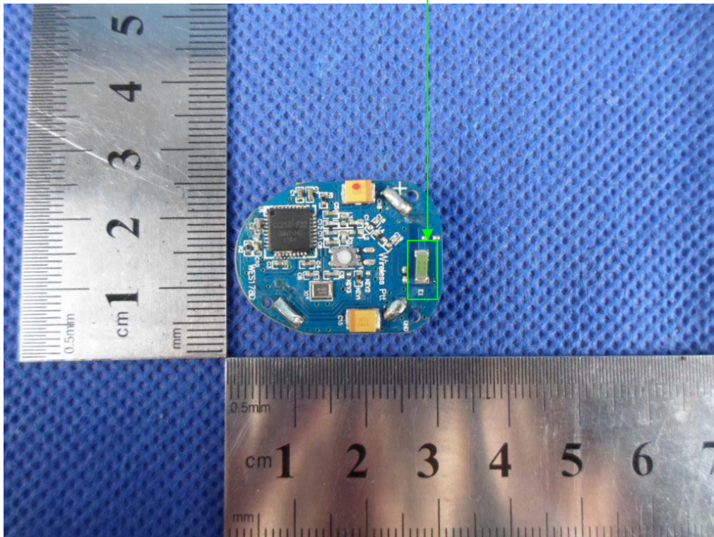
Photo 9 Antenna
