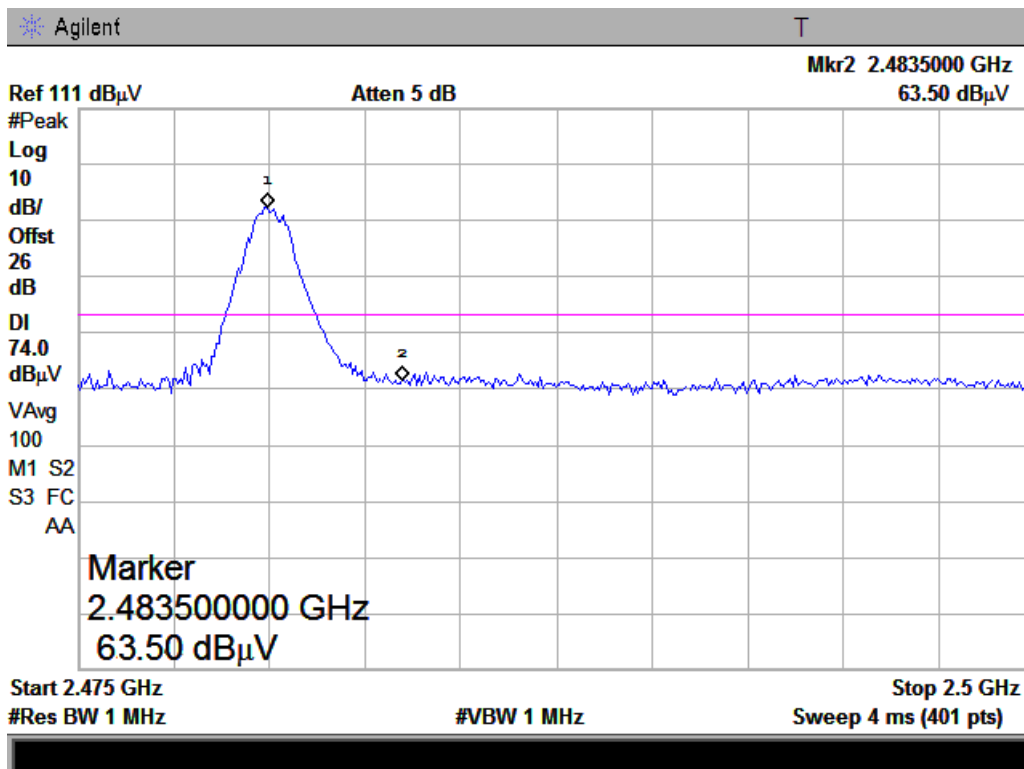
(Plot 8: Channel = 78, Detector Mode: Peak)
