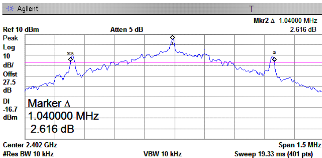
(Plot 3A: Channel = 0)
