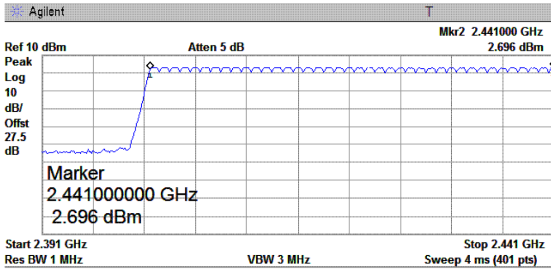
(Plot 1: 2391MHz to 2441MHz)
