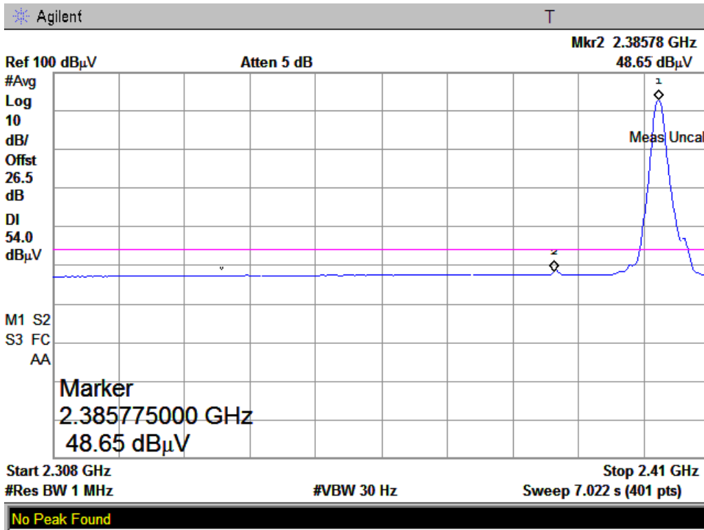
(Plot 5: Channel = 0, Detector Mode: Average)
