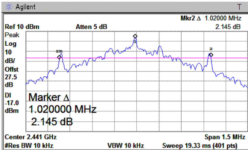
(Plot 3B: Channel = 39)
