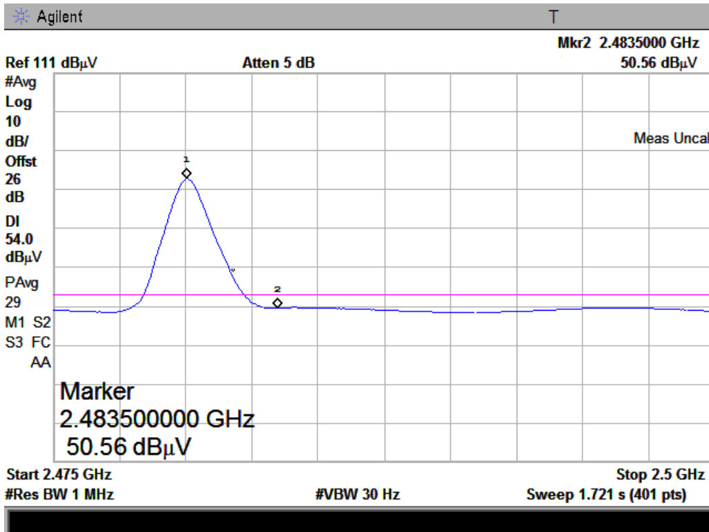
(Plot 7: Channel = 78, Detector Mode: Average)
