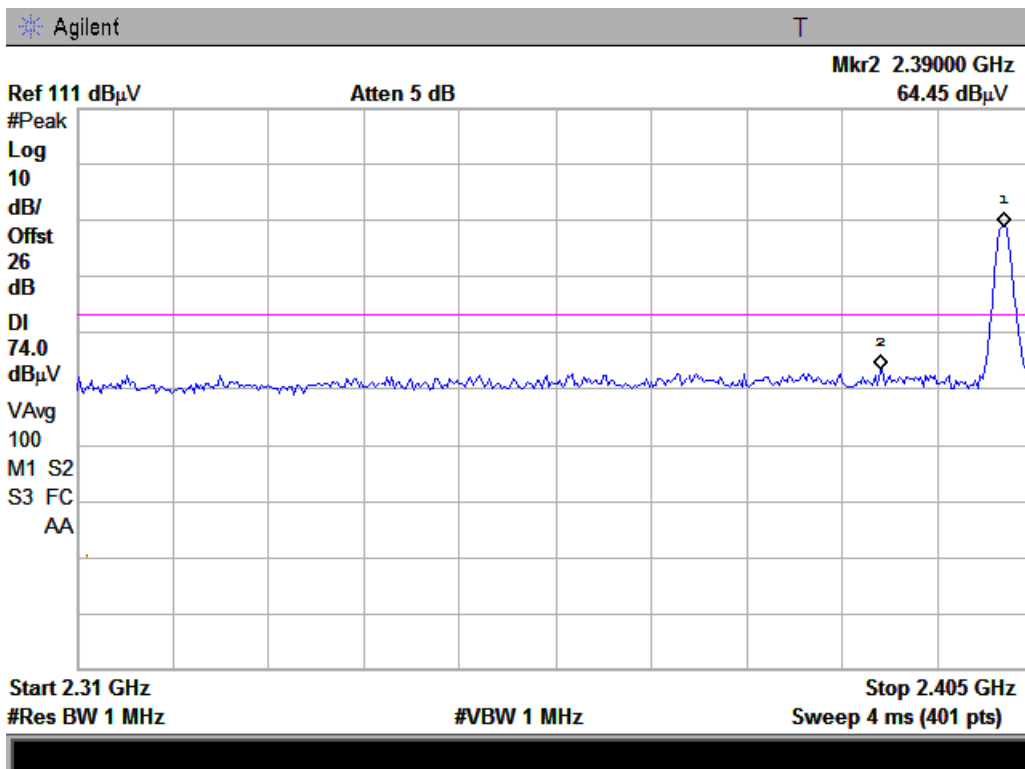
(Plot 6: Channel = 0, Detector Mode: Peak)
