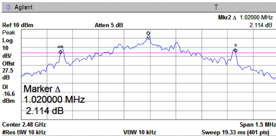
(Plot 3C: Channel = 78)
