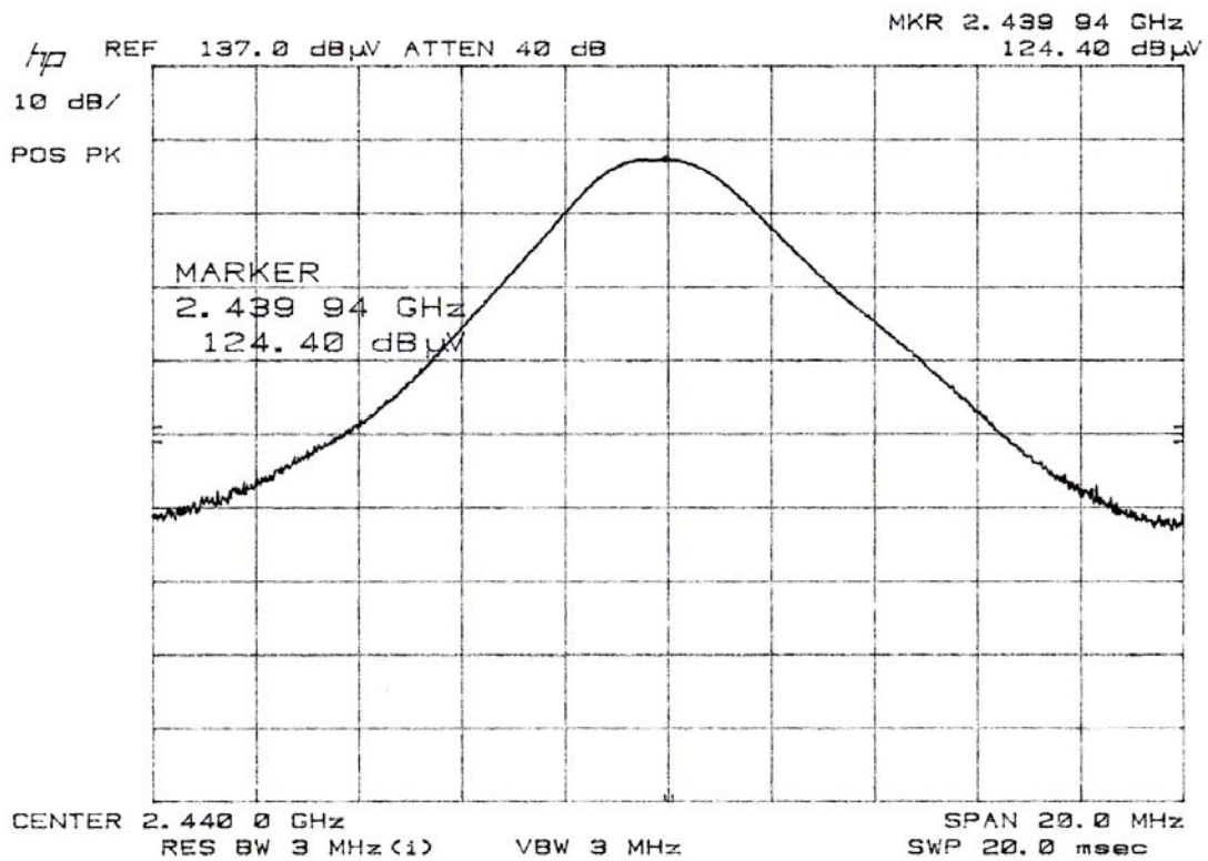
Plot 8: Peak Output Power - Middle Channel 2440 MHz Level
