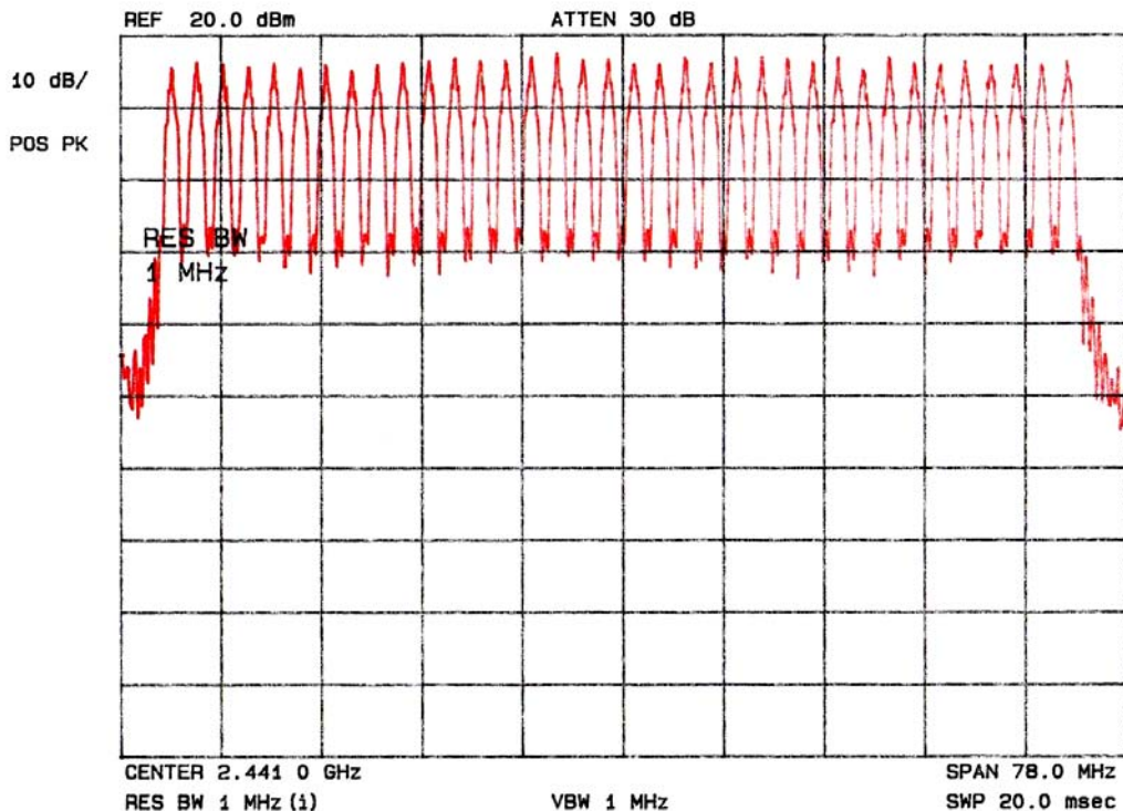
Plot 20: Number of Hopping Frequencies – Test Mode Command A
