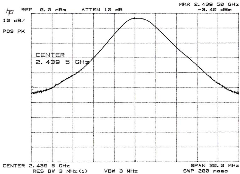
Plot 2: Radiated Spurious Emission - Middle Channel 2440 MHz Level (-3.4dBm = 103.6dBuV)
