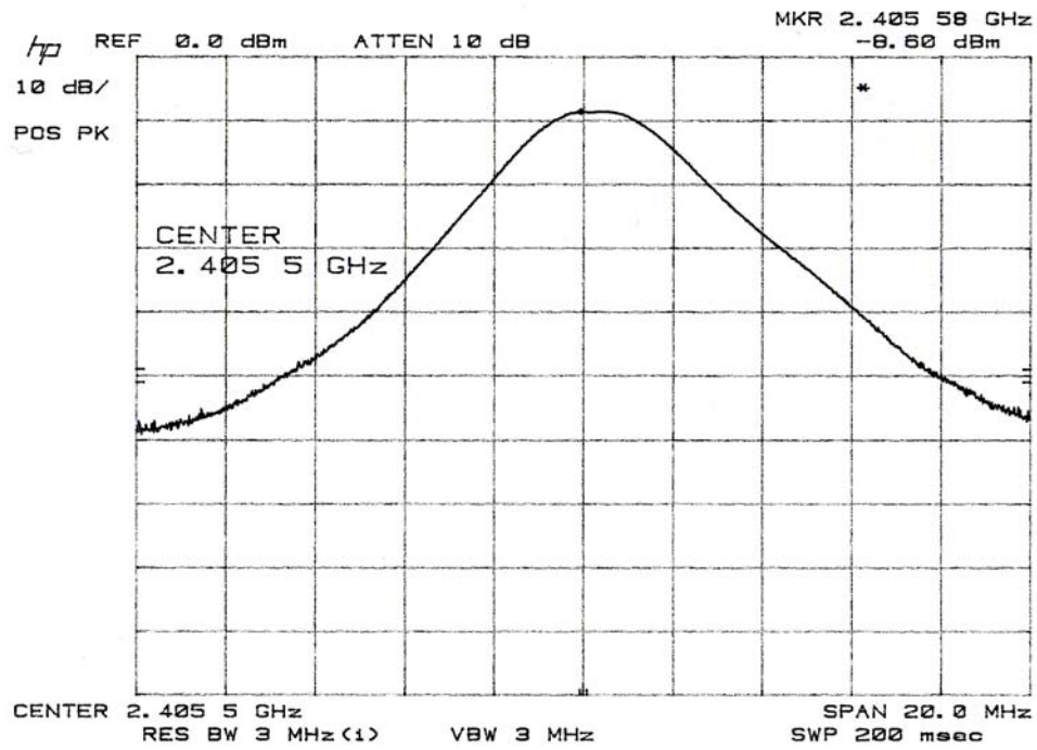
Plot 1: Radiated Spurious Emission - Low Channel 2406 MHz Level (-8.6dBm = 98.4dBuV)
