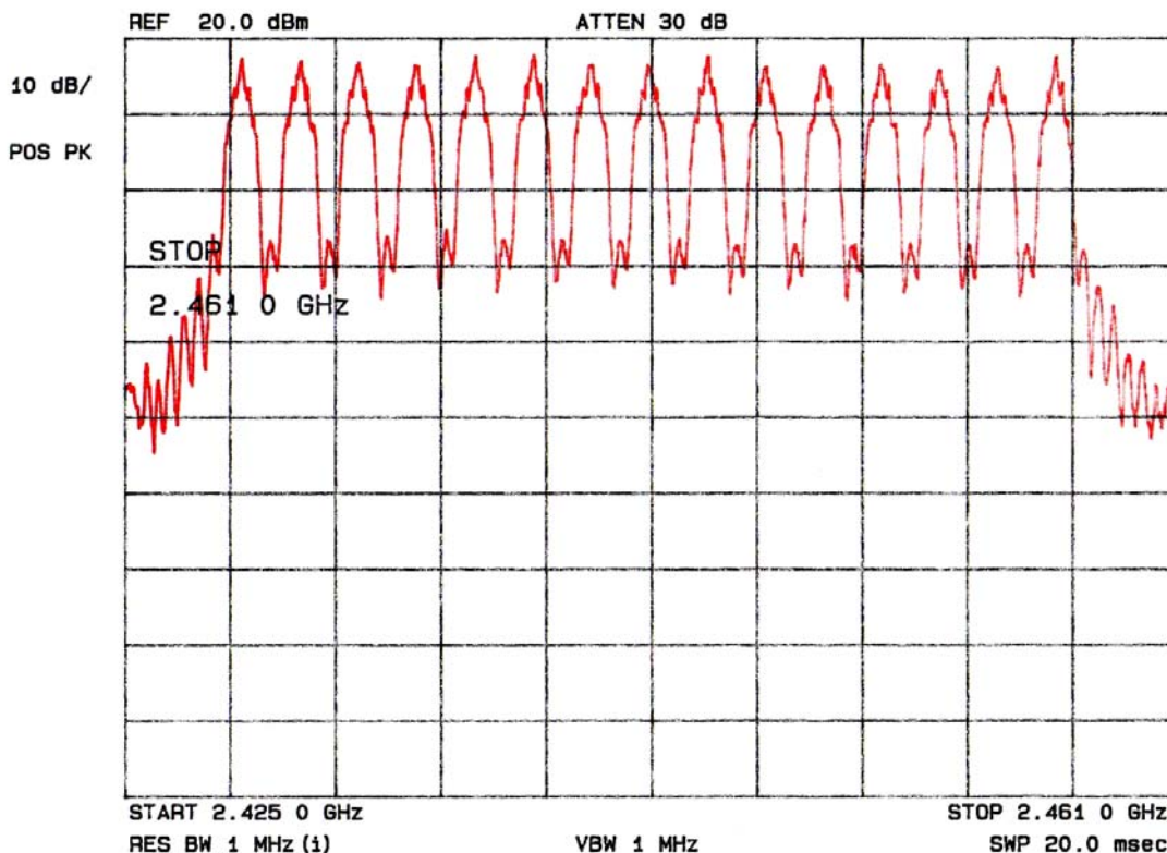
Plot 25: Number of Hopping Frequencies - Command F
