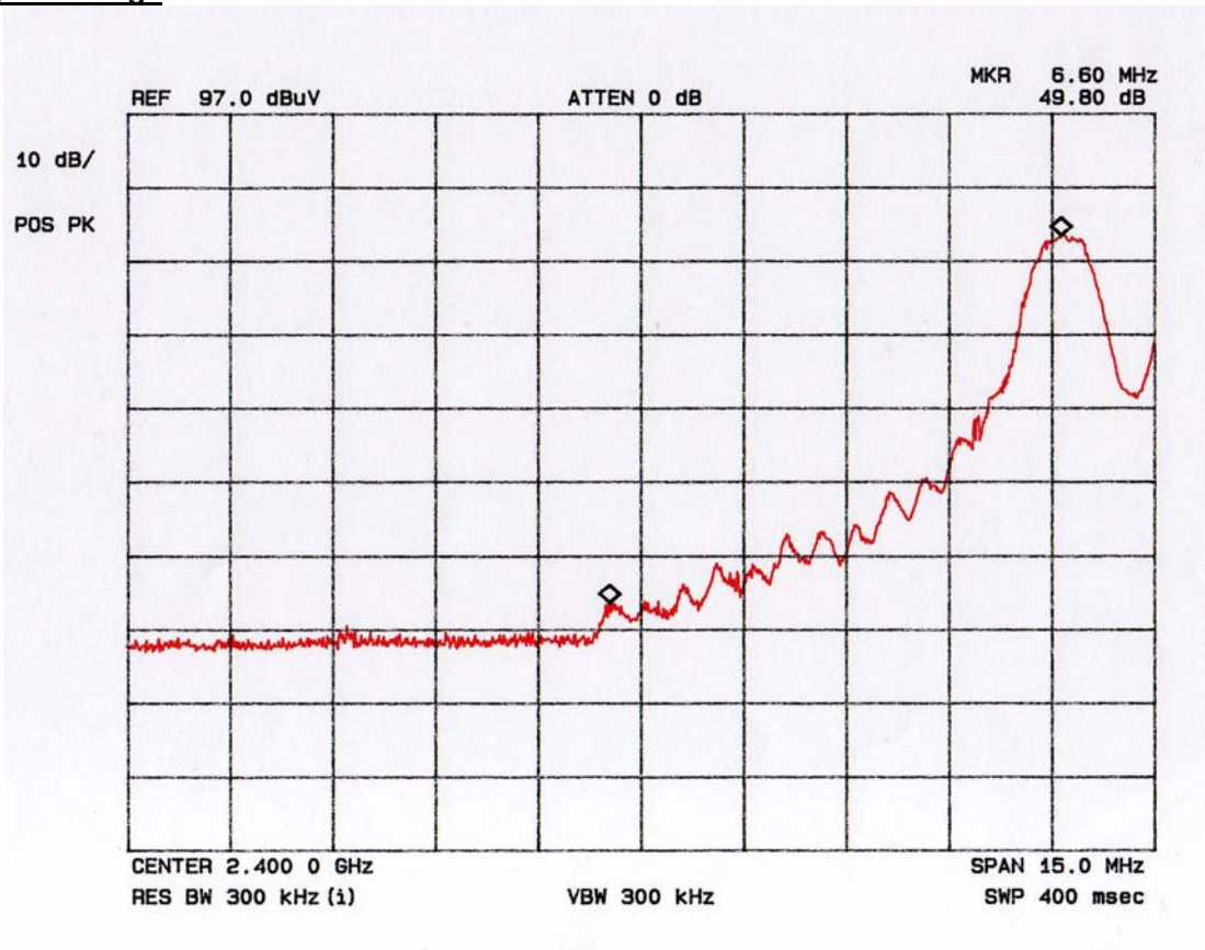
Plot 10: Low Channel Bandedge
