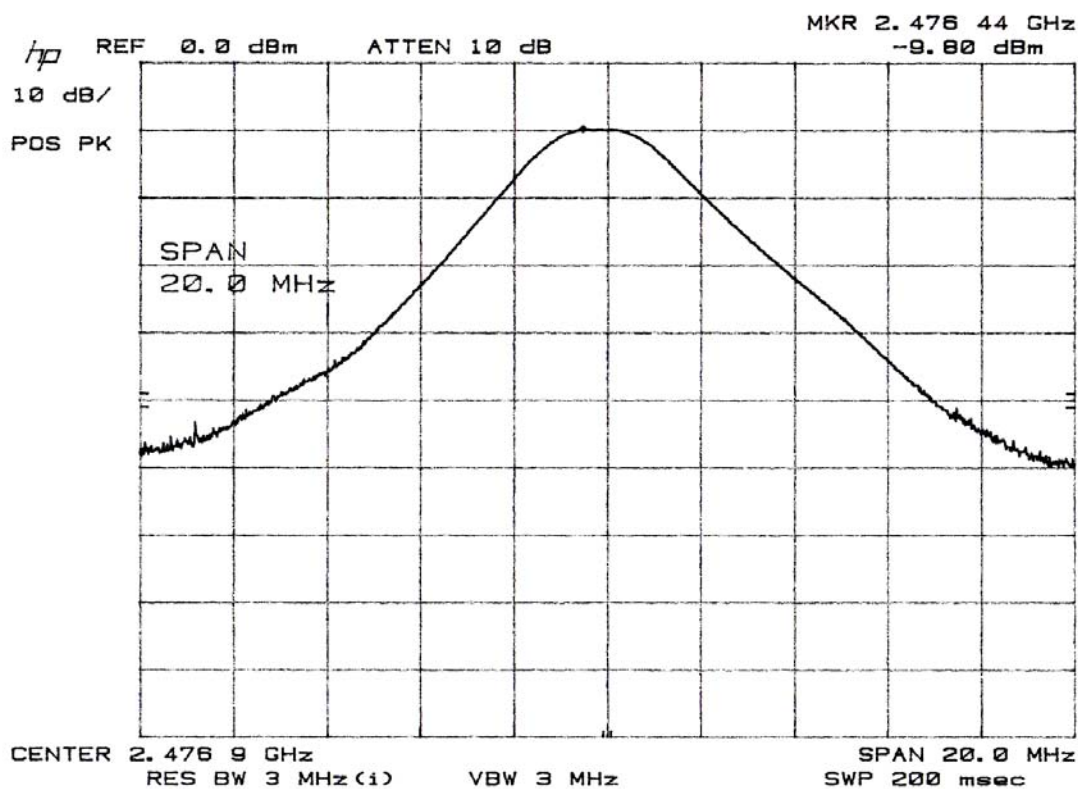
Plot 3: Radiated Spurious Emission - High Channel 2477 MHz Level (-9.8dBm = 97.2dBuV)
