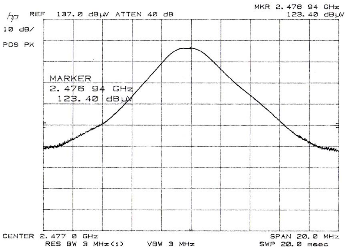
Plot 9: Peak Output Power - High Channel 2477 MHz Level
