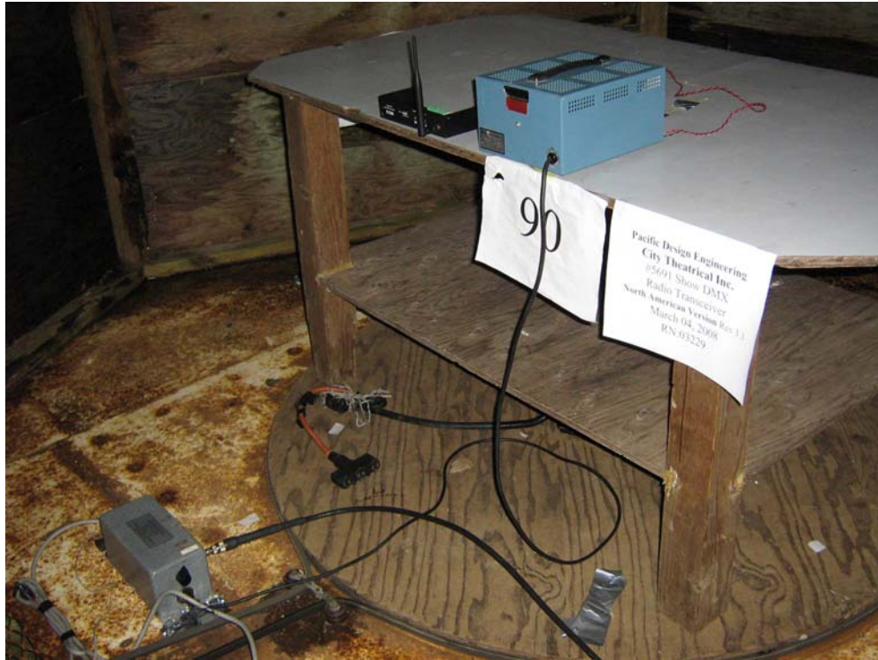
City Theatrical Inc. ShoW DMX Radio Transceiver-#5691 North American Version AC Conducted set-up-Figure 4
