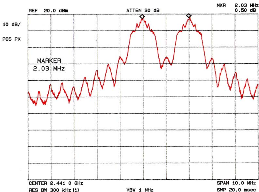
Plot 15: Hopping Channel Carrier Frequency Separation
