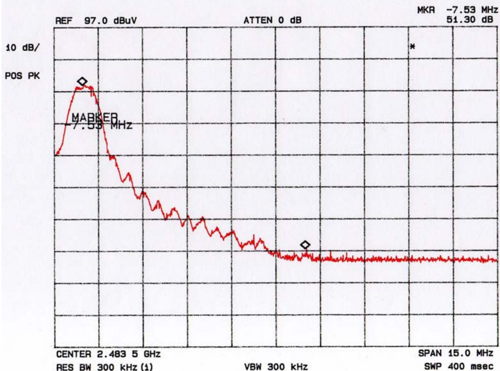
Plot 11: High Channel Bandedge
