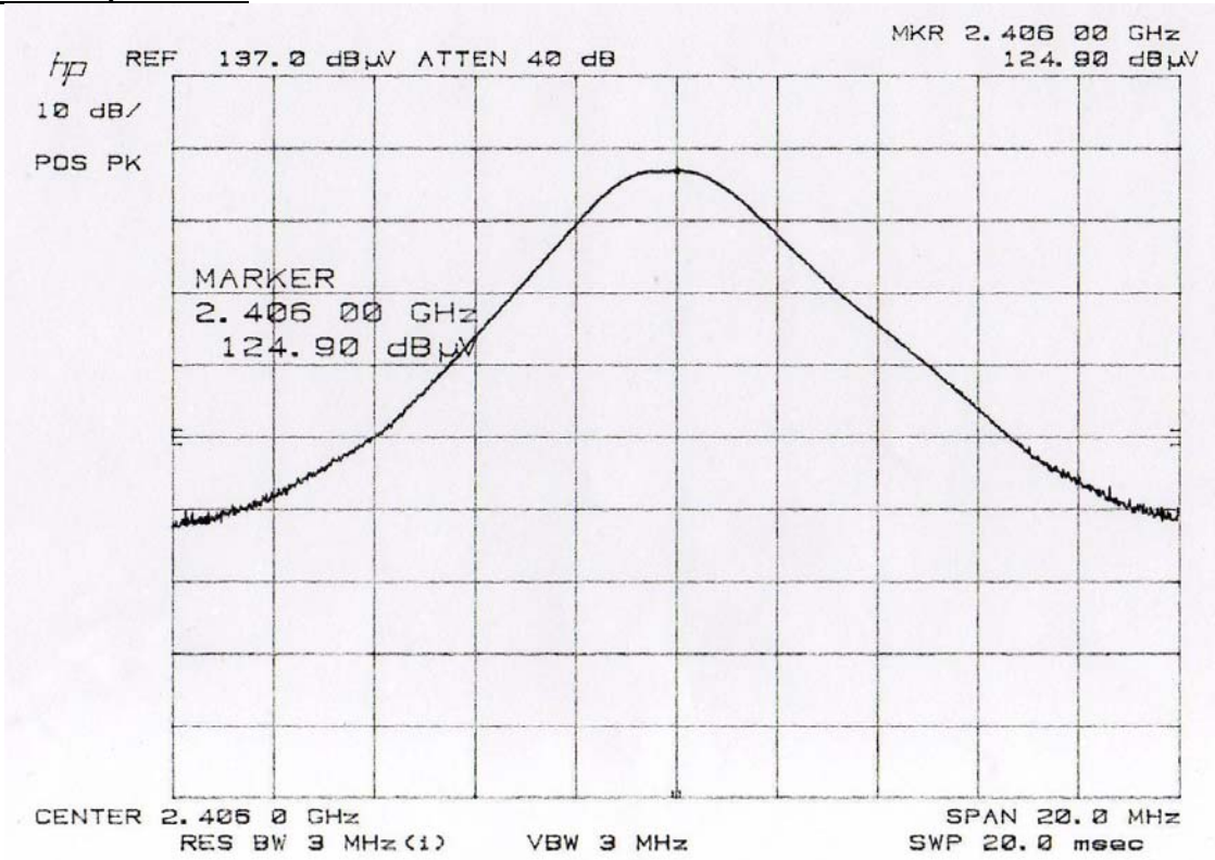
Plot 7: Peak Output Power - Low Channel 2406 MHz Level
