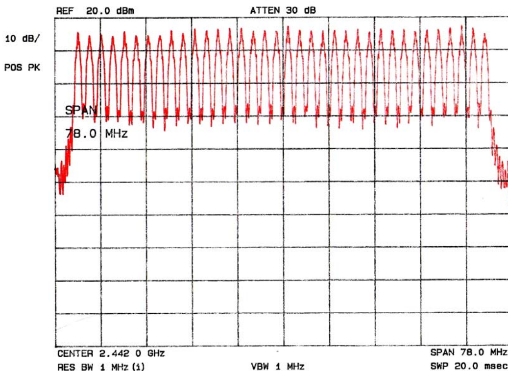
Plot 21: Number of Hopping Frequencies - Test Mode Command B
