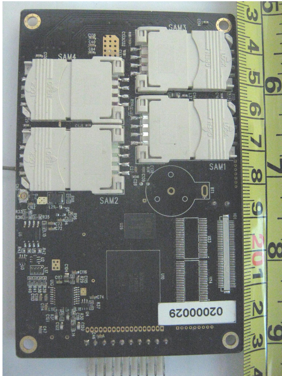
Main-Board PCB View 1
