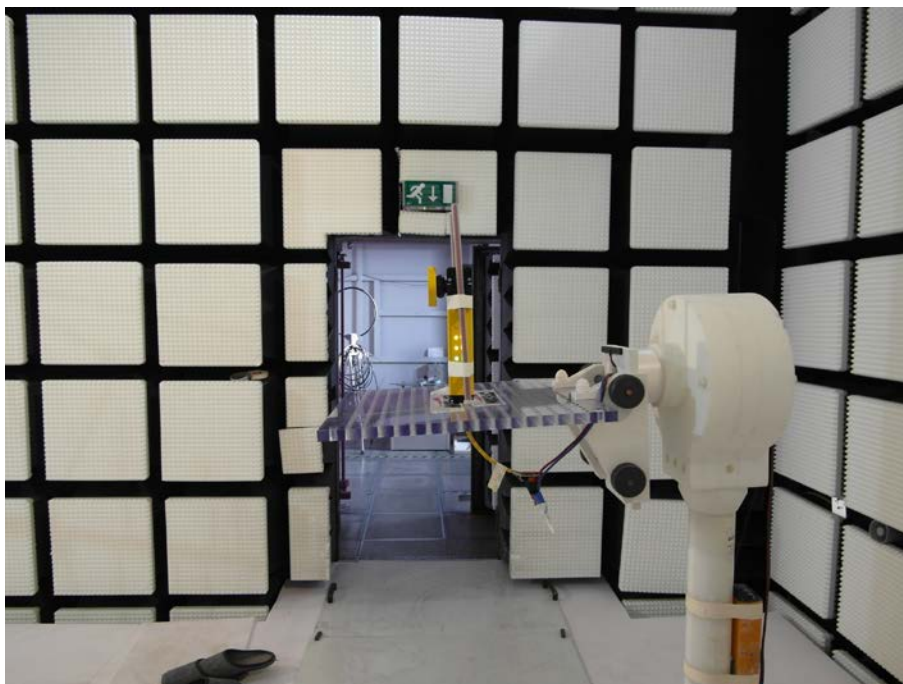
Photo 2: Test setup for radiated emissions
