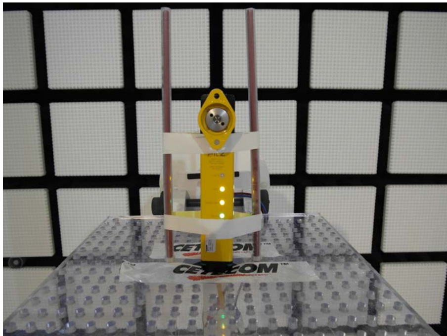
Photo 5: Test setup for radiated emissions
