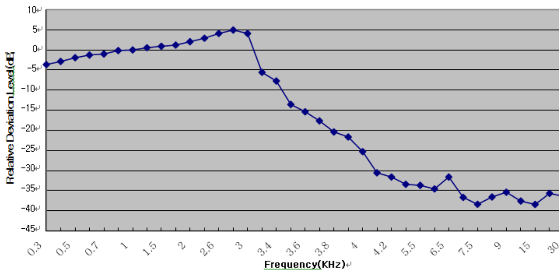
Audio Frequency Response
