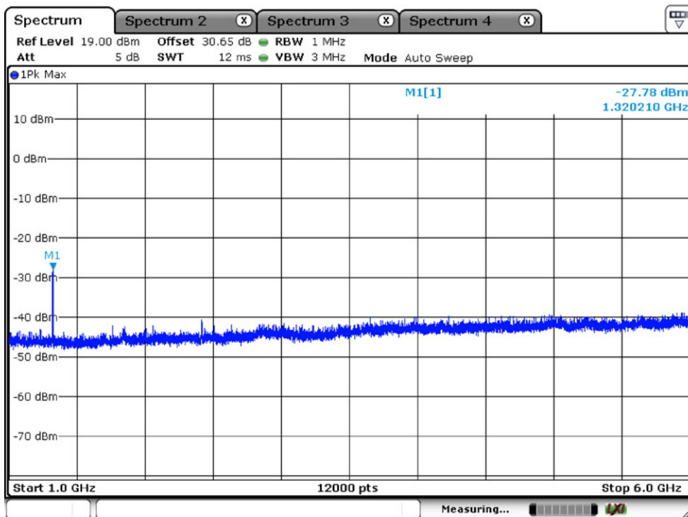
1 GHz – 6 GHz, Spacing Channel 12.5 kHz, 440.0125 MHz
