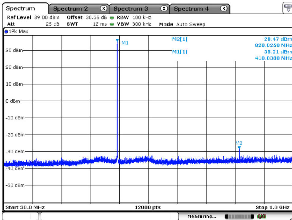
30 MHz – 1 GHz, Spacing Channel 12.5 kHz, 410.0125 MHz
