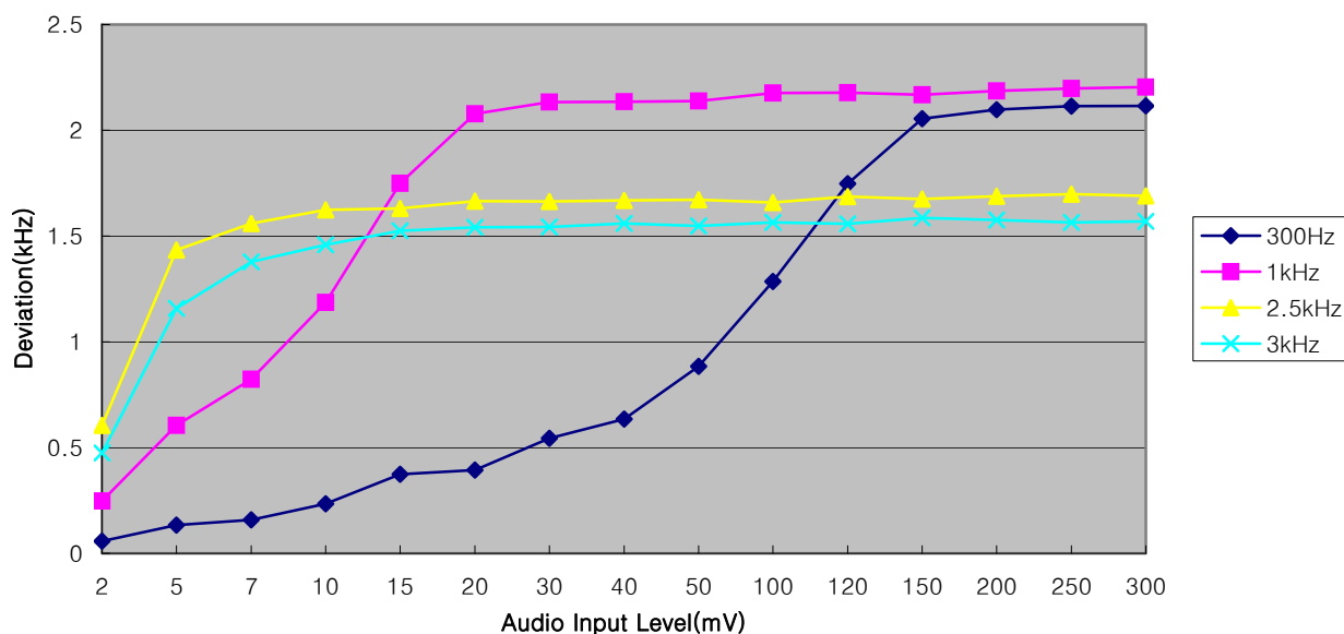
Deviation Limiting
