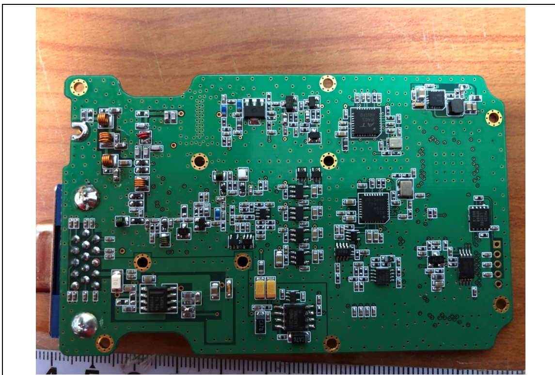
MainBoard-Rear
