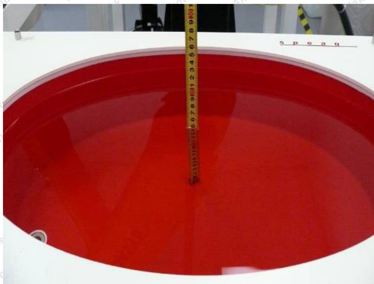
Photograph of the depth in the Head Phantom (150MHz, 15.3cm)
