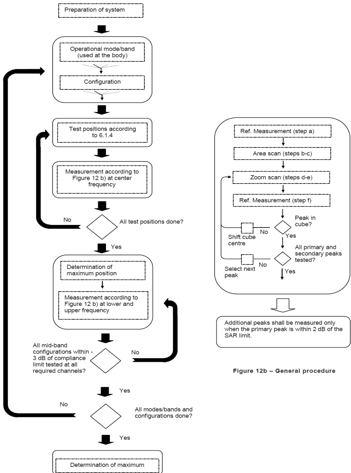
Figure 12a – Tests to be performed
