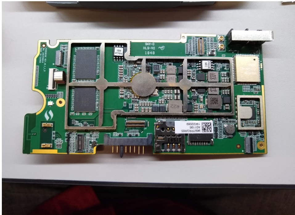
main PCBA (back) without shields
