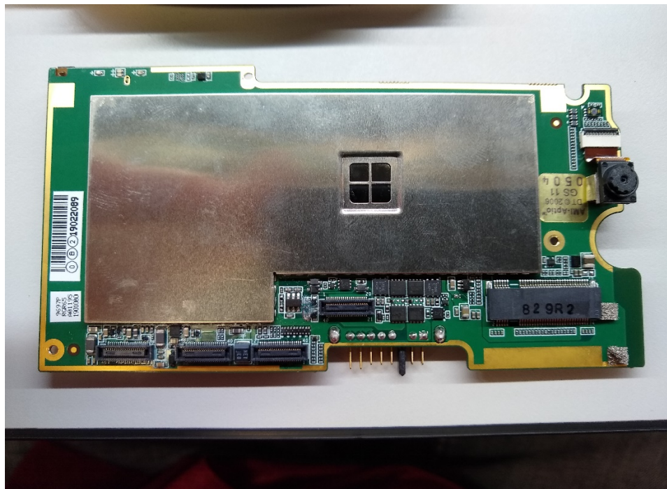
main PCBA (front) with shields
