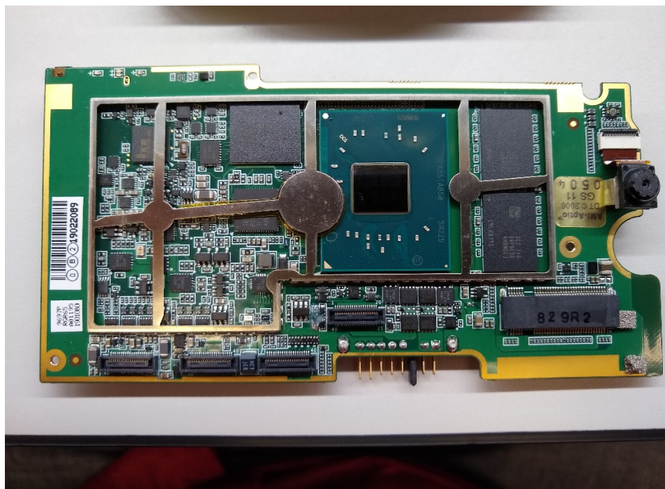
main PCBA (front) without shields
